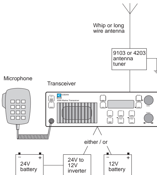
Figure 2.2 A typical ship station installation
