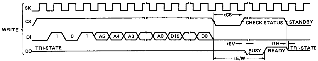
Fig. 18 NMC9346 ROM Write Timing Chart
