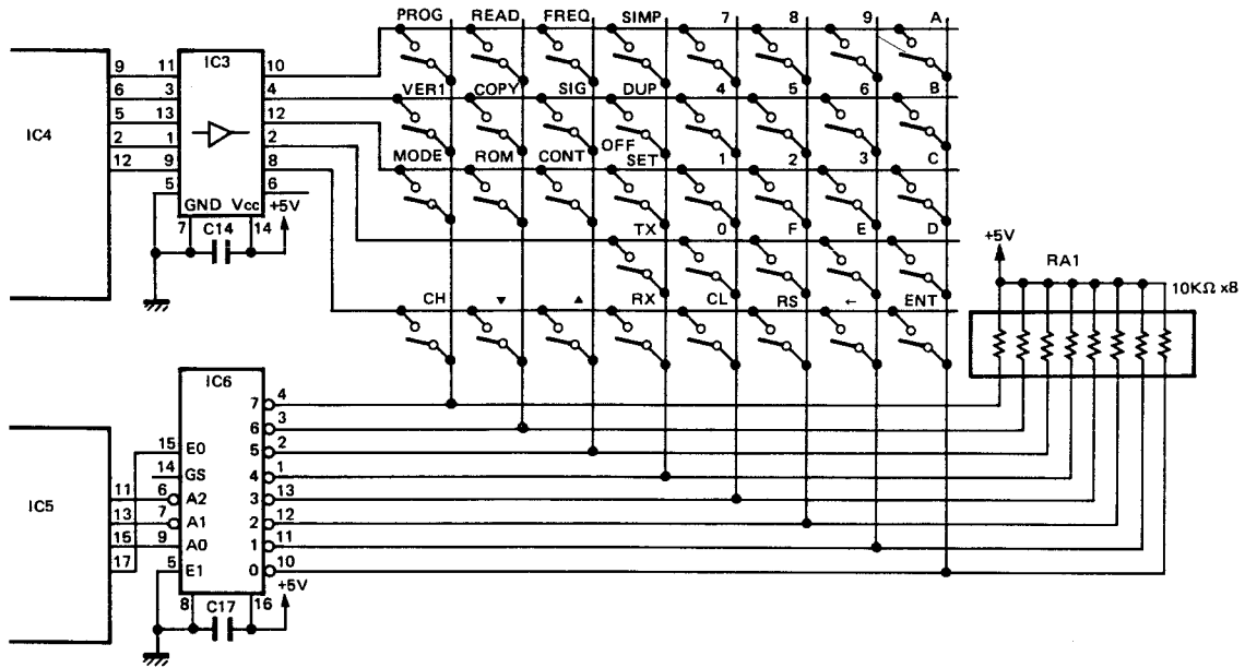
Fig. 23 Keyboard Interface Circuit Block Diagram
