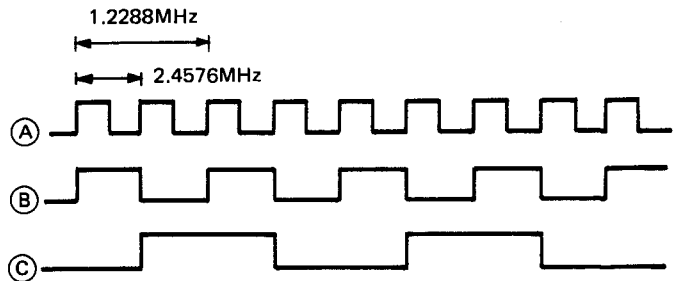
Fig. 12 Clock Circuit Timing Chart
