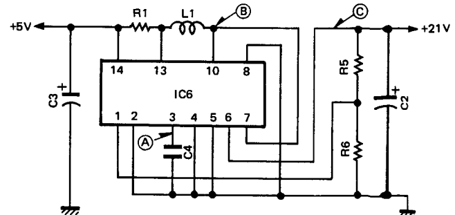
Fig. 9 + 21V Power Supply Circuit Block Diagram
