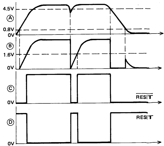
Fig. 14 Reset Circuit Timing Chart
