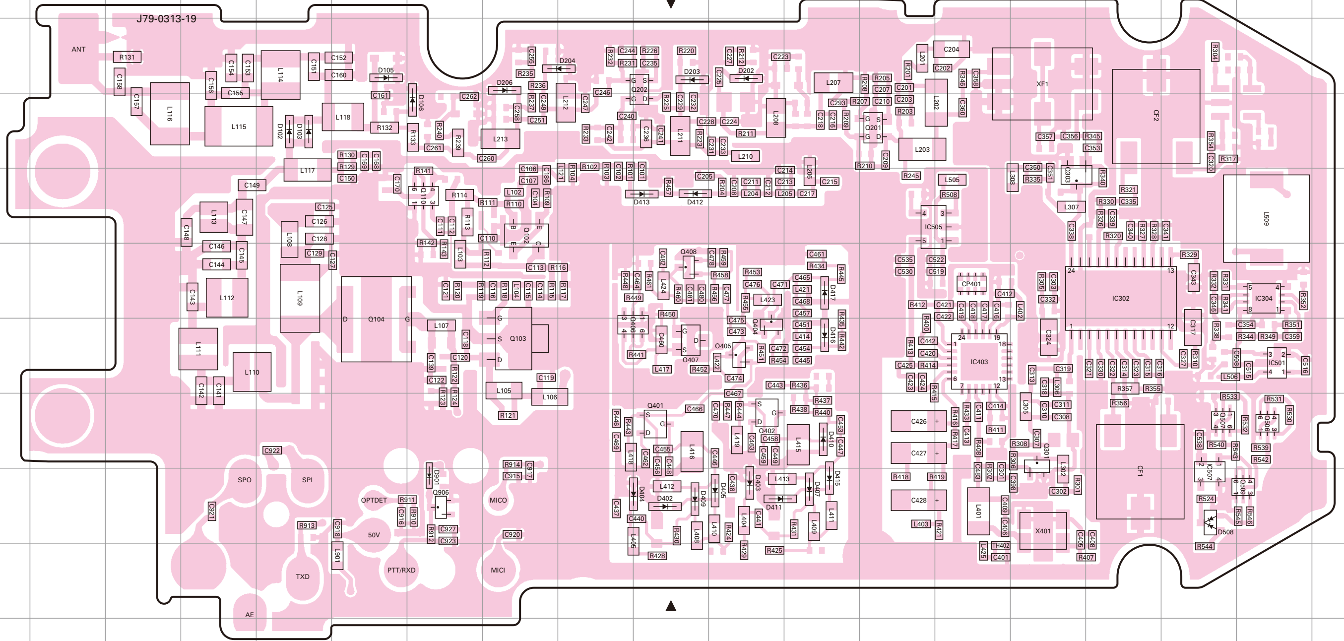
TX-RX UNIT (X57-8040-10) Foil side view (J79-0313-19)
