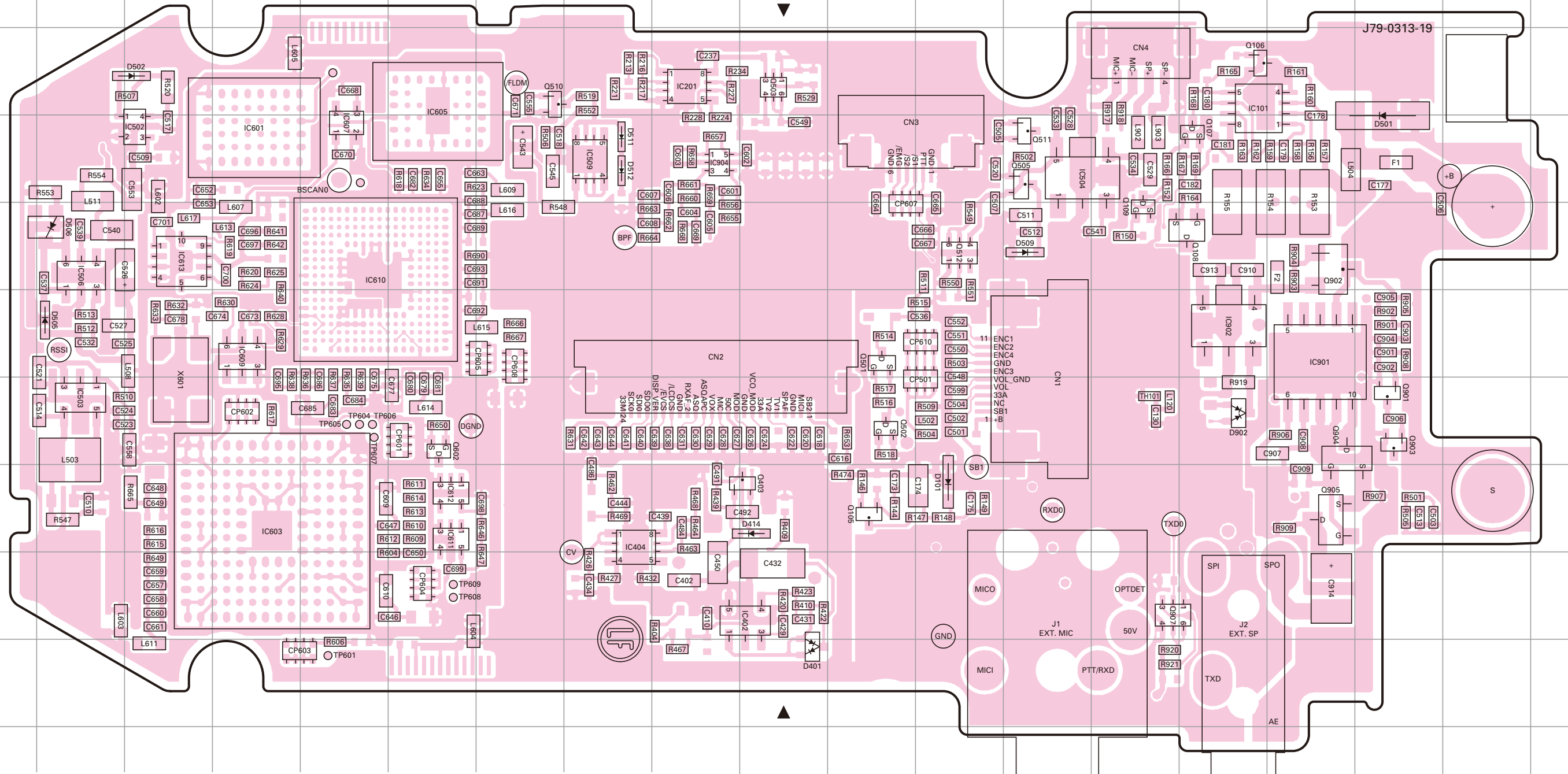
TX-RX UNIT (X57-8040-10) Component side view (J79-0313-19)
