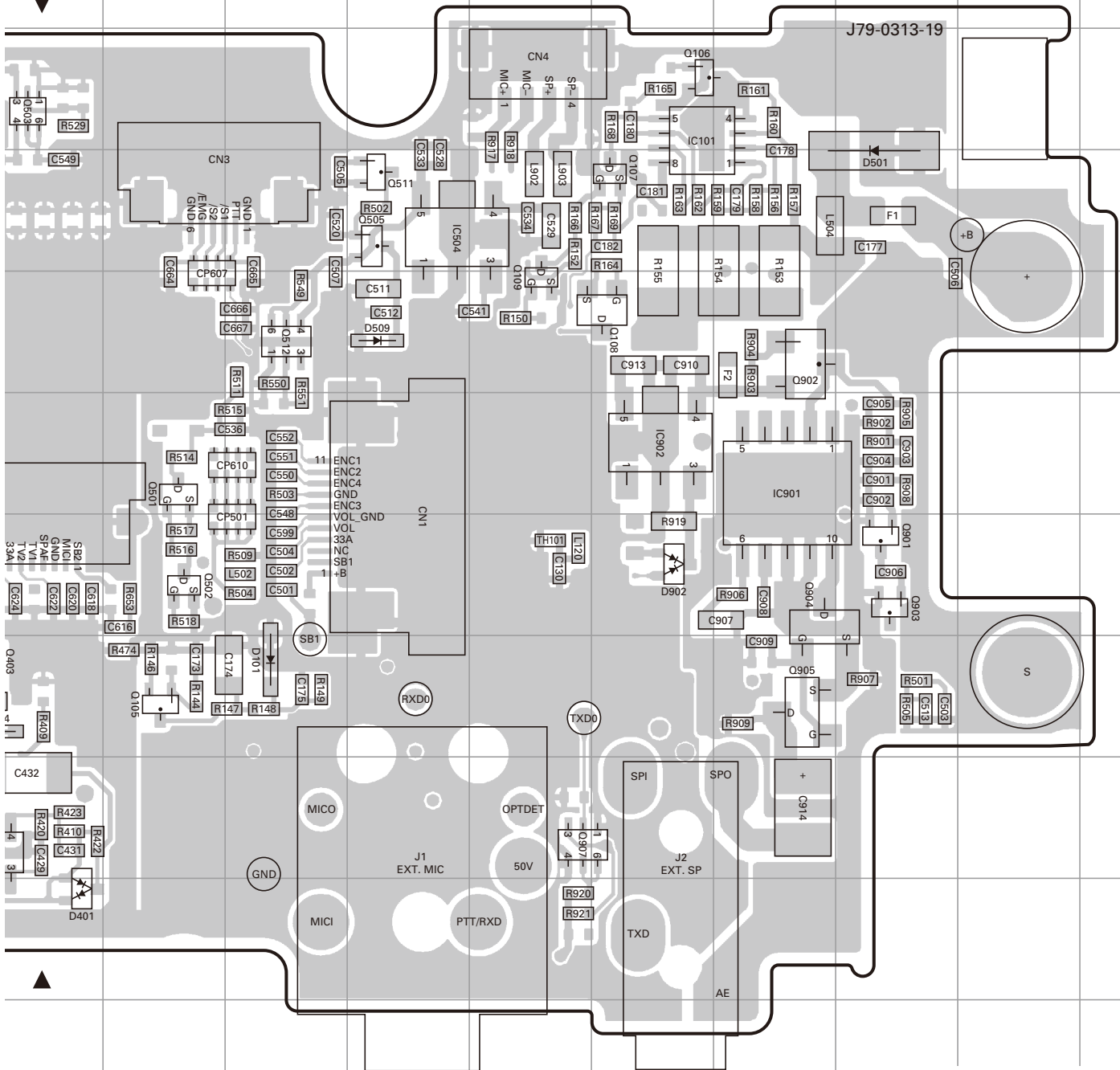
TX-RX UNIT (X57-8040-10) Component side view (J79-0313-19)
