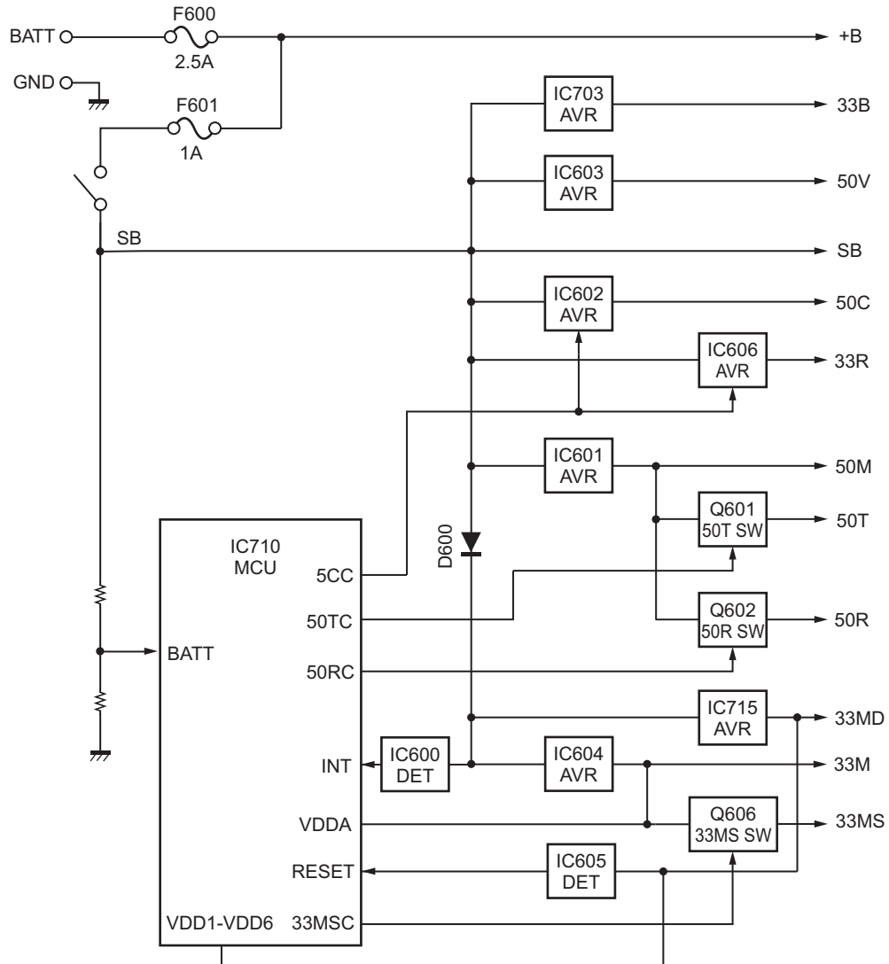
Fig.9 Power supply
