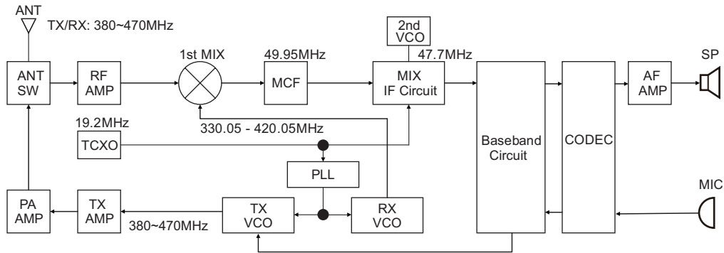
Fig.1 Frequency configuration
