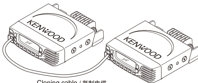
Cloning cable / 复制电缆 (E30-3382-05)
