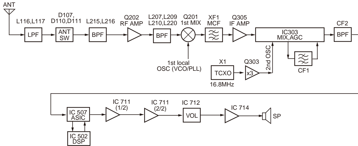
Fig.2 Receiver System / 图 2 接收机系统
