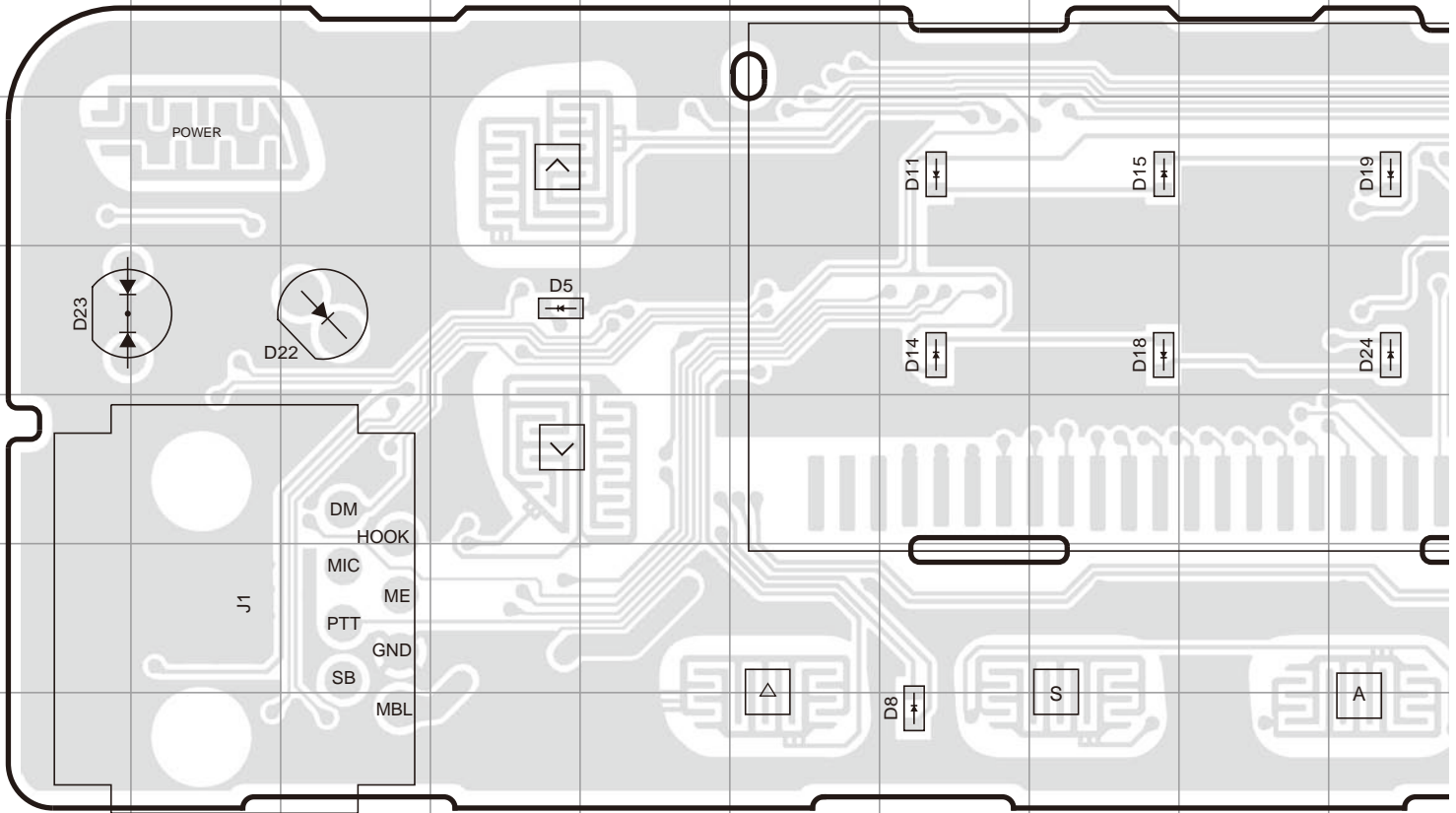
DISPLAY UNIT (X54-3830-10) Component side view (J79-0345-09)
