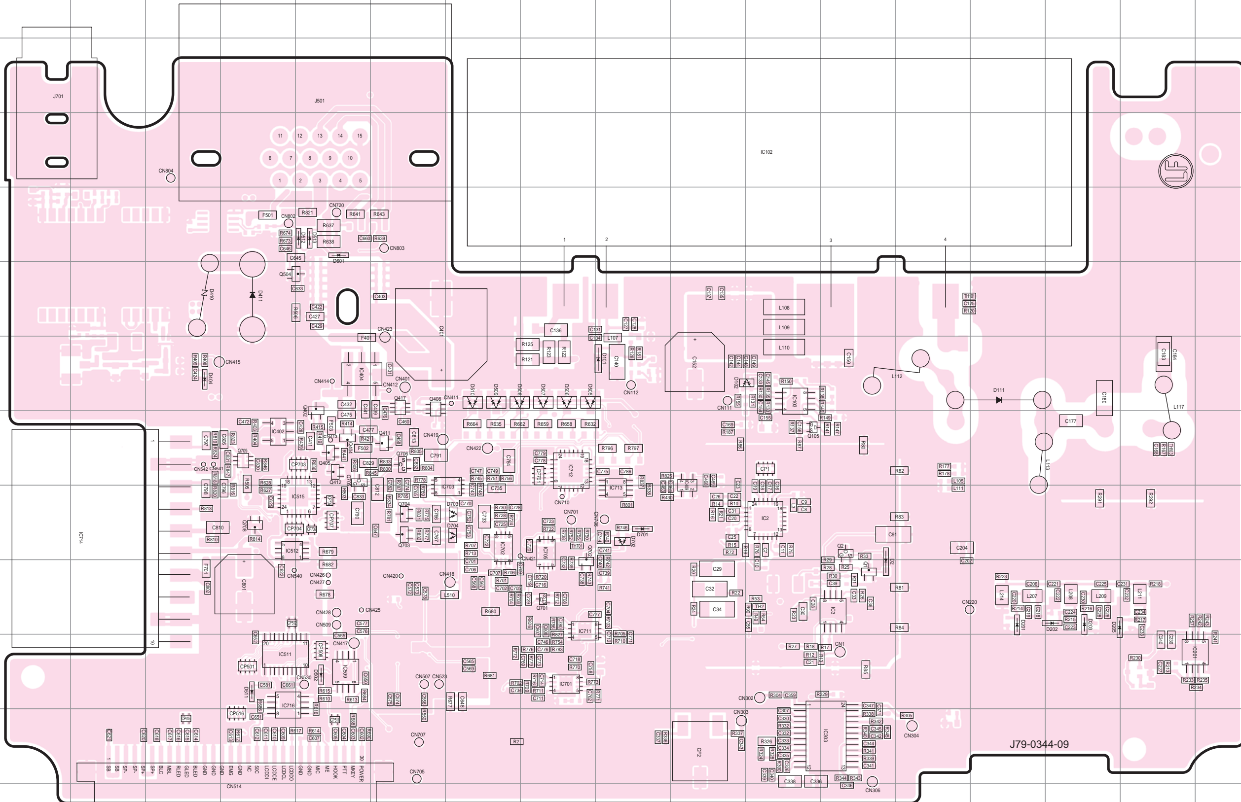
TX-RX UNIT (X57-8240-13) Component side view (J79-0344-09)
