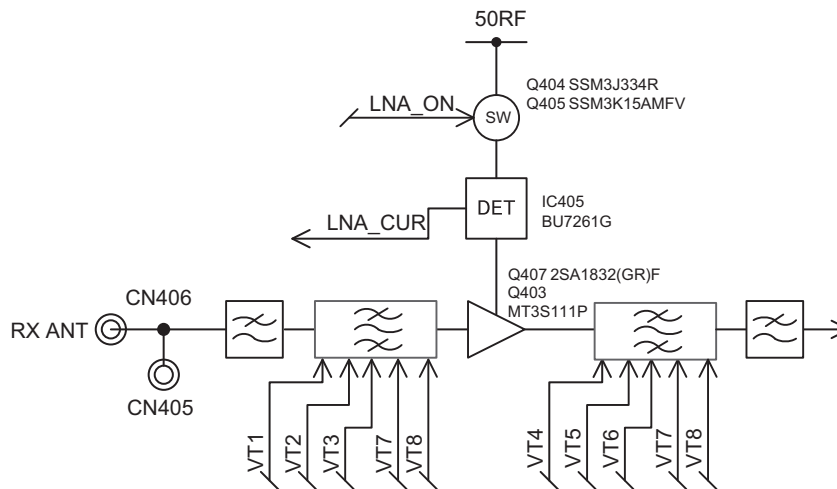
Fig.11 Front-end circuit
