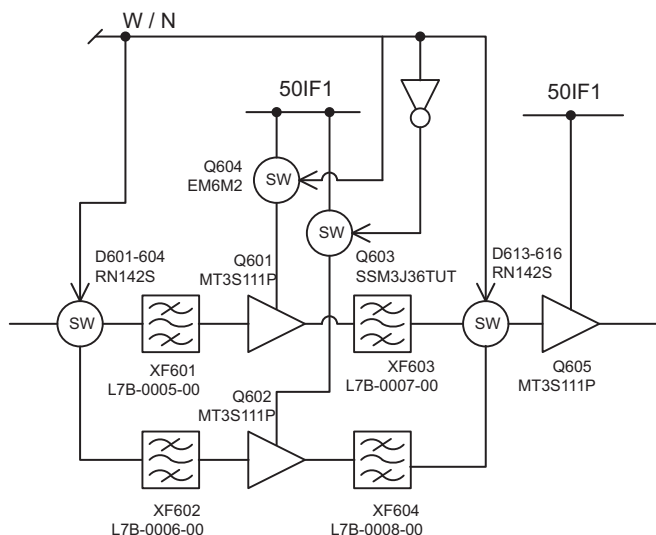
Fig.13 1st-IF circuits
