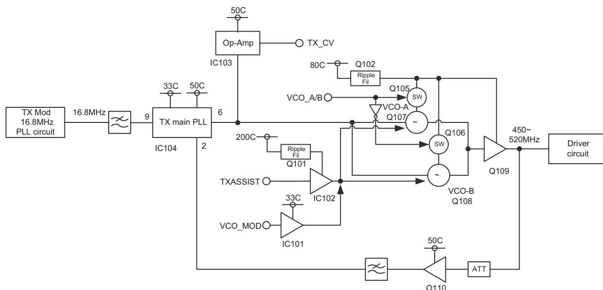
Fig.5 Transmitter main PLL circuit
