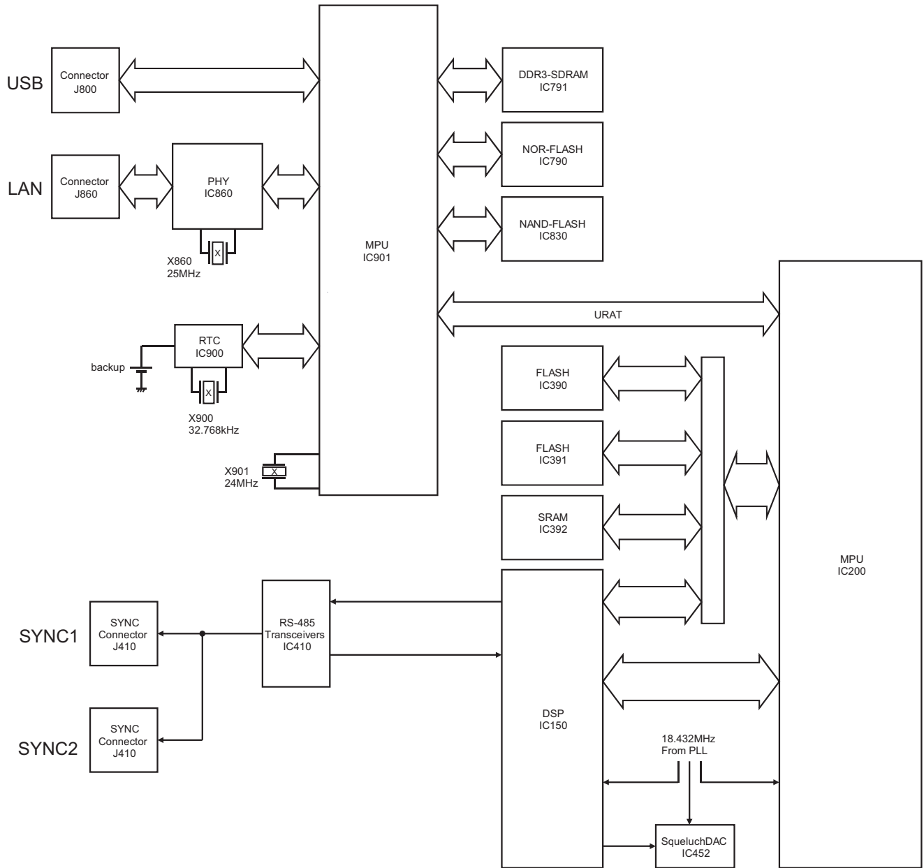
Fig.17 Control circuit
