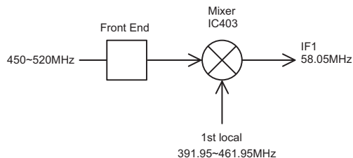
Fig.12 1st-Mixer circuit
