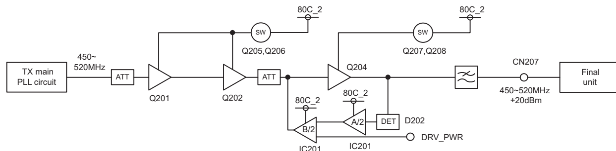
Fig.6 Driver circuit
