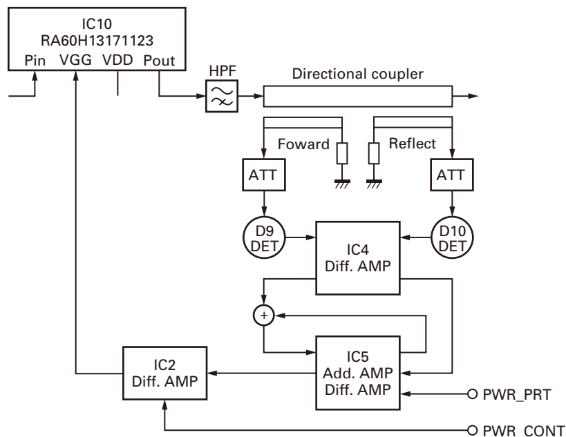
Fig. 11 APC circuit
