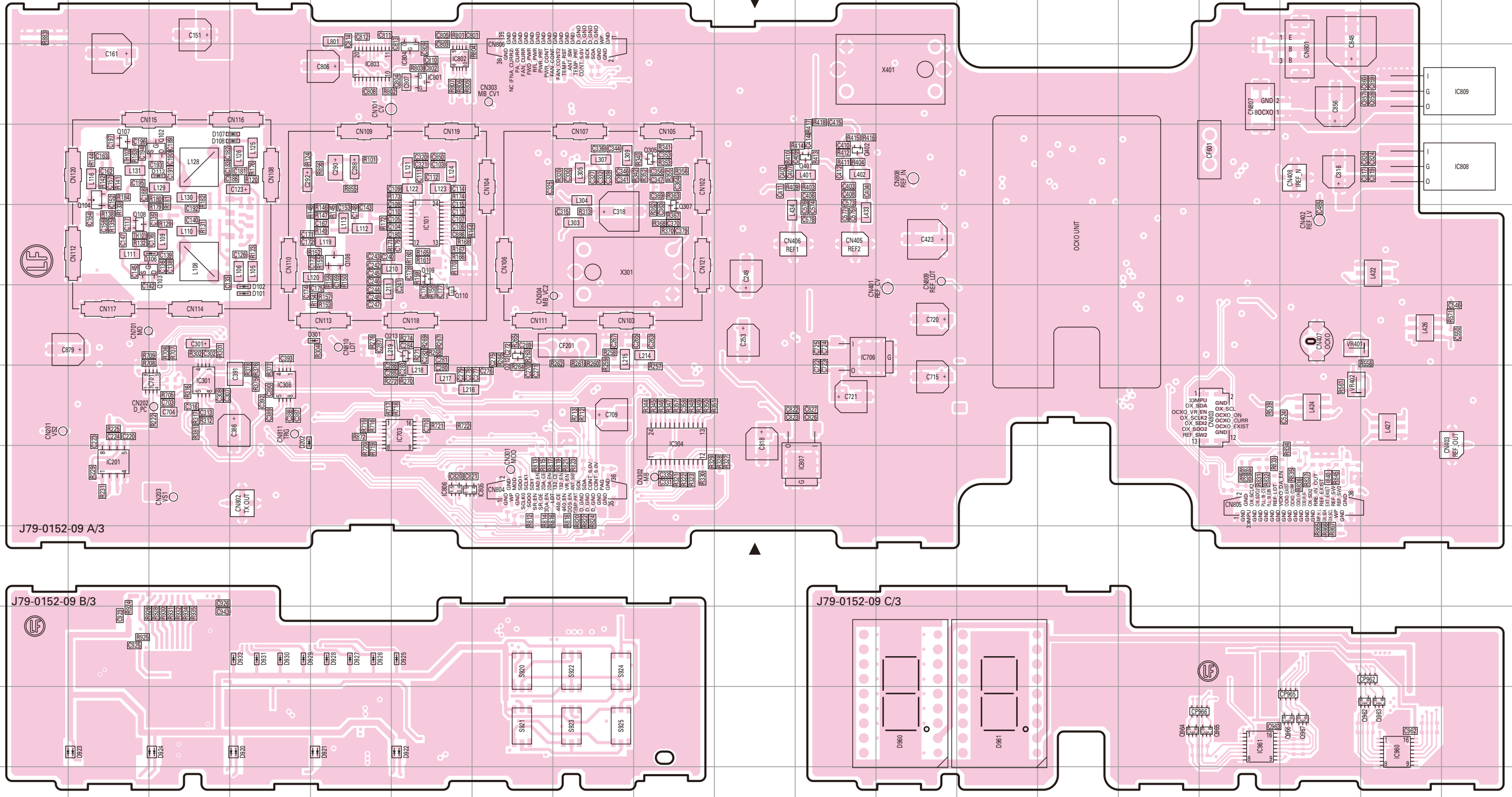
TX UNIT (X56-3112-71) Component side view (J79-0152-09)
