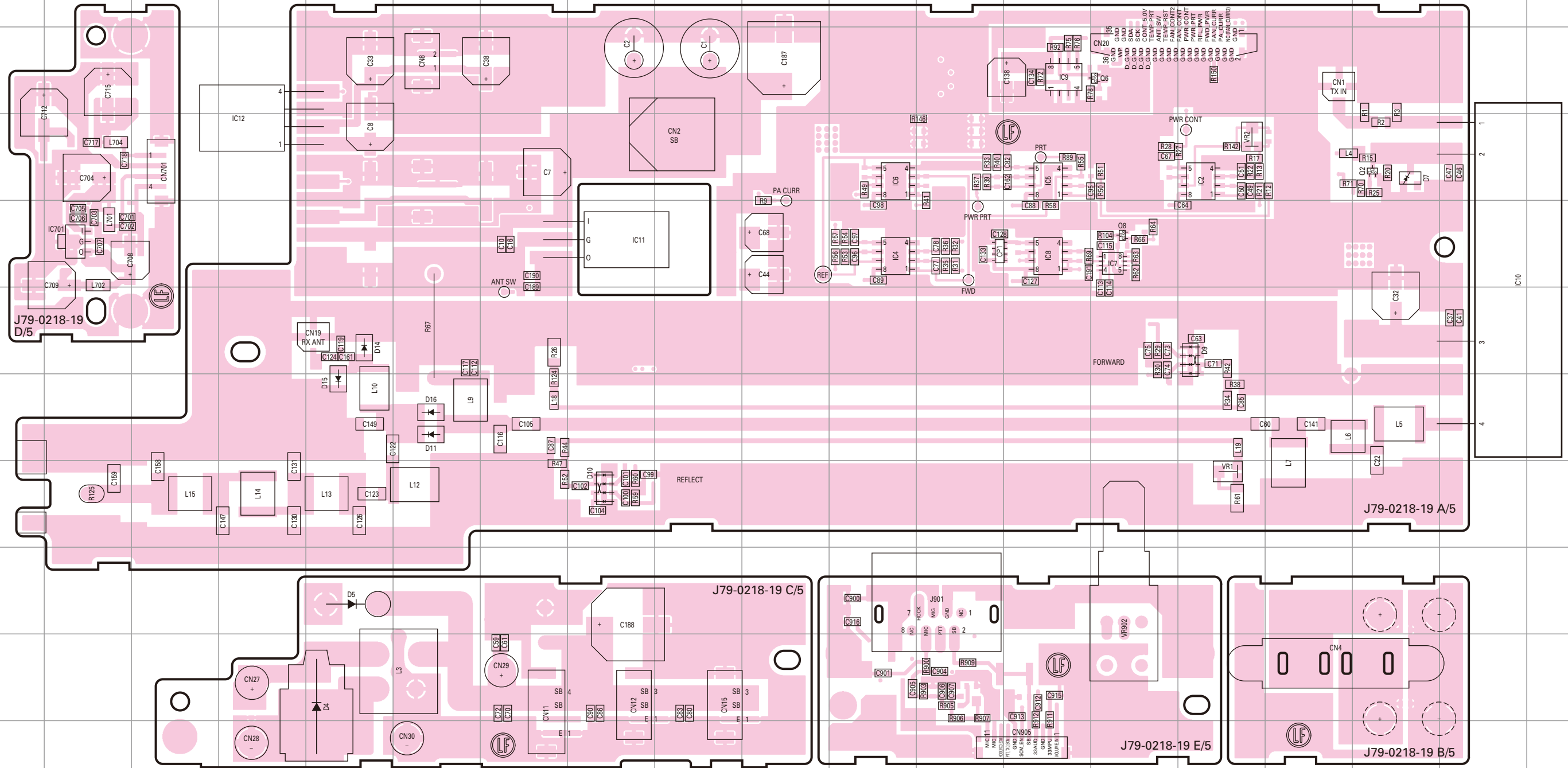
FINAL UNIT (X45-3852-70) Component side view (J79-0218-19)
