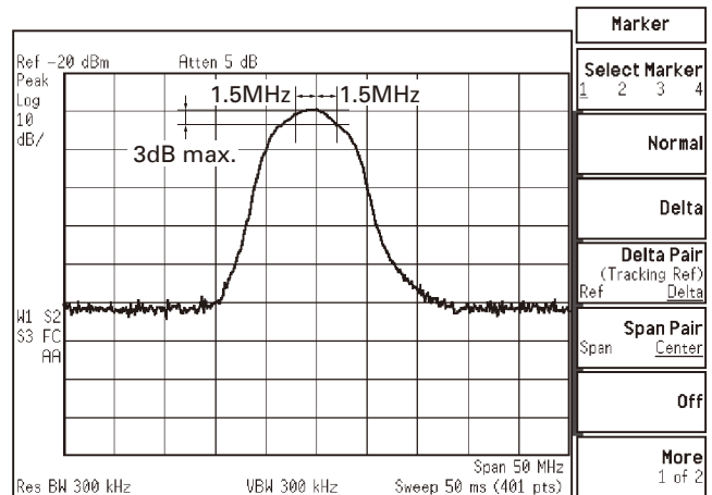
BPF center frequency (Production default) E: 160.1MHz Pass bandwidth: \pm 1.5 MHz at 3dB
