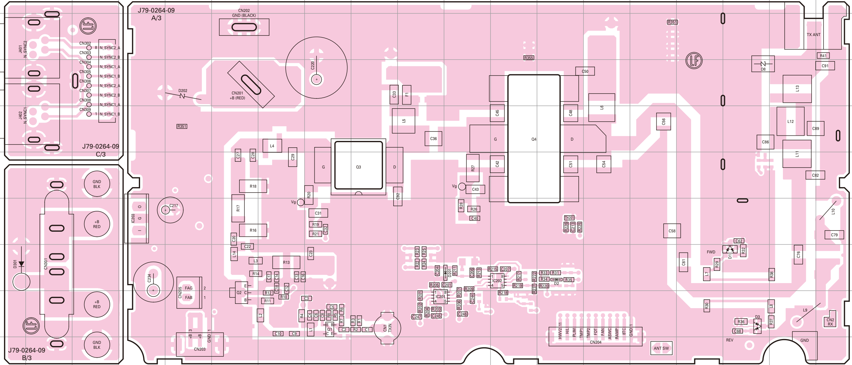
FINAL UNIT (X45-3930-10) Component side view (J79-0264-09)
