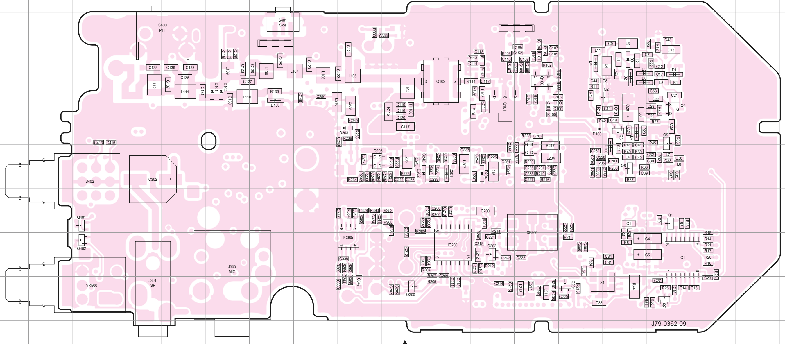
TX-RX UNIT (X57-8092-71) Foil side view (J79-0362-09)
