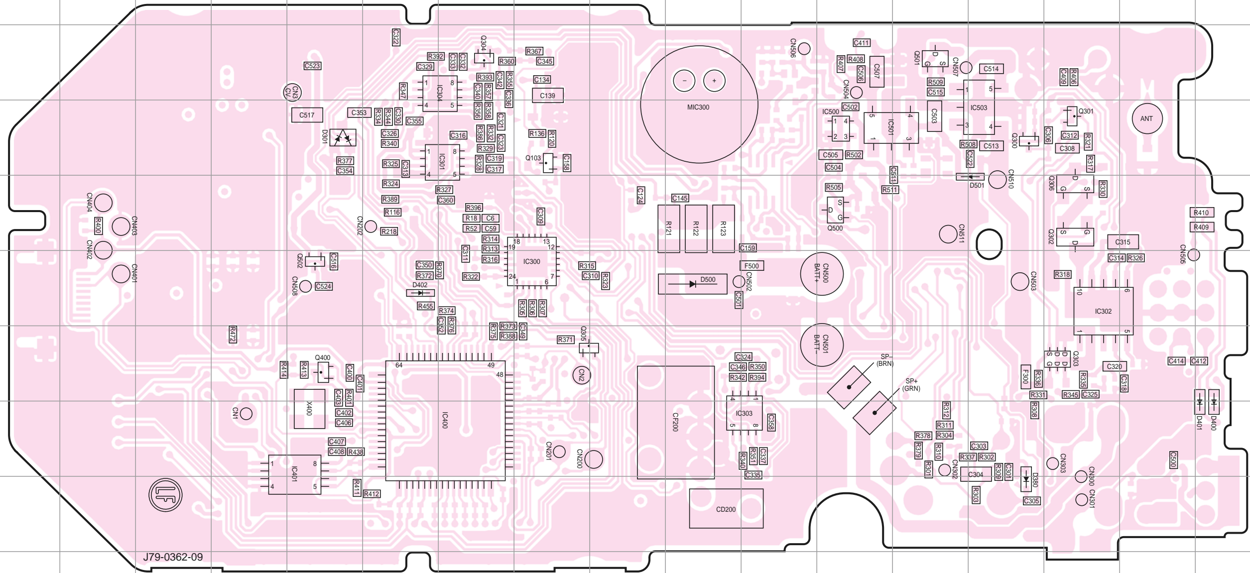
TX-RX UNIT (X57-8092-71) Component side view (J79-0362-09)
