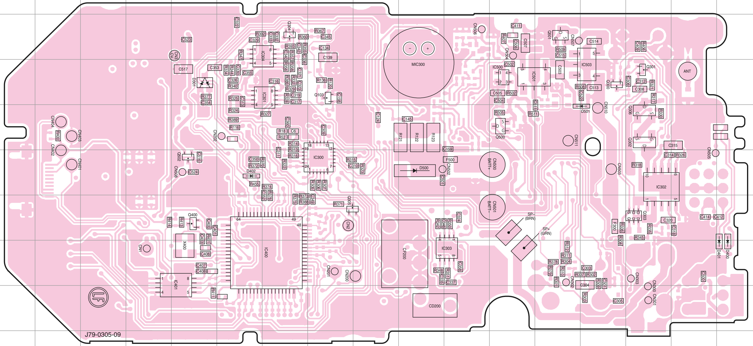
TX-RX UNIT (X57-8093-00) Component side view (J79-0305-09)
