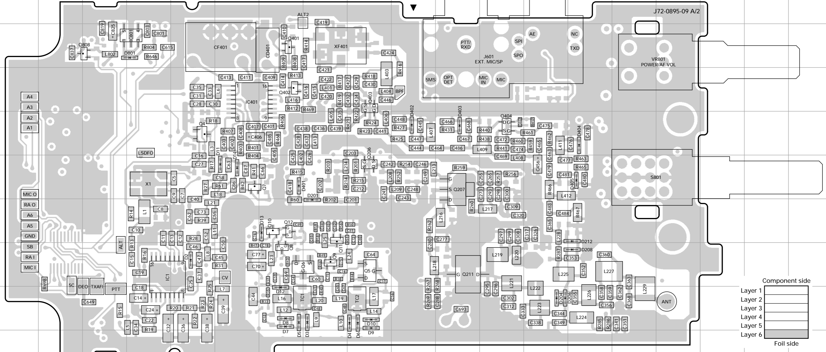
TX-RX UNIT (X57-6722-71) Foil side view (J72-0895-09)
