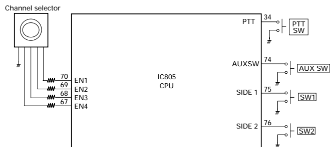
Fig. 13 Control system
