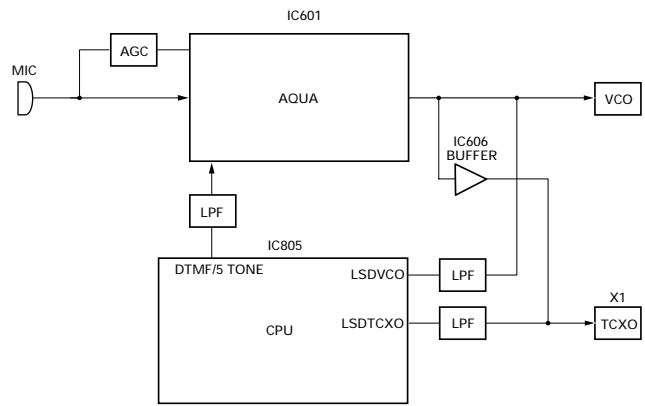
Fig. 8 Microphone amplifier
