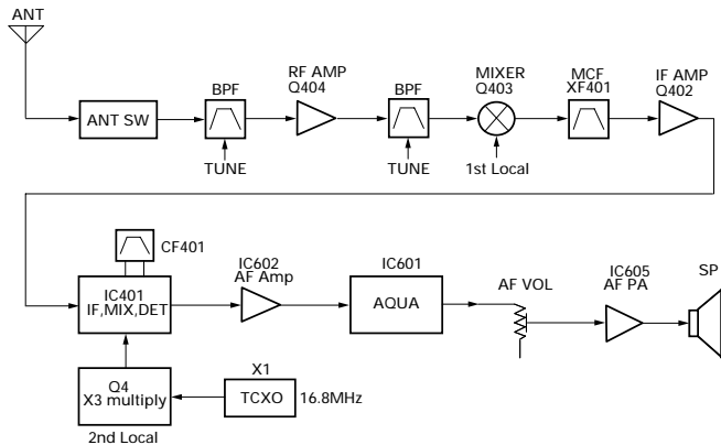
Fig. 2 Receiver section
