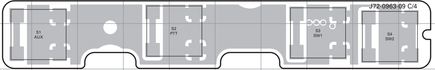
TX-RX UNIT (X57-7000-XX) (C/4) -10 : K -11 : K2 Component side view (J72-0963-09 C/4)
