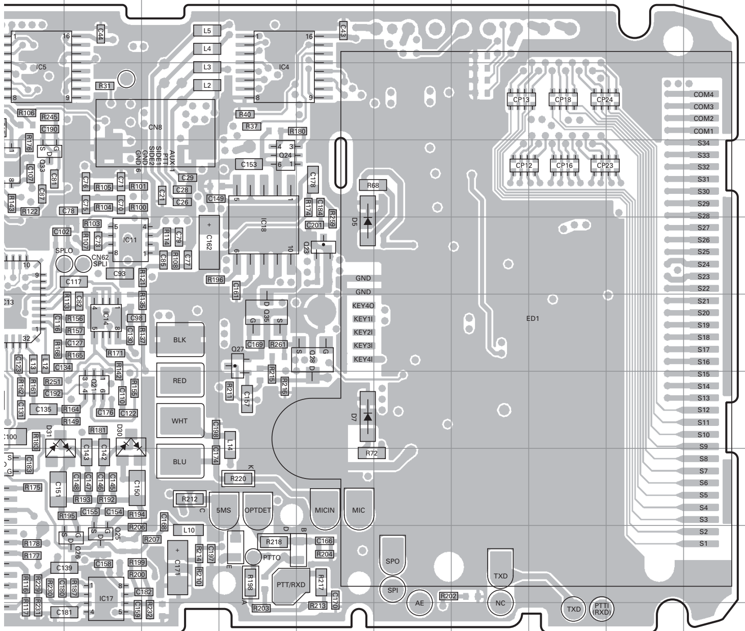
TX-RX UNIT (X57-7000-XX) (B/4) -10 : K -11 : K2 Component side view (J72-0963-09 B/4)
