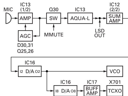
Fig. 5 Microphone amplifier
