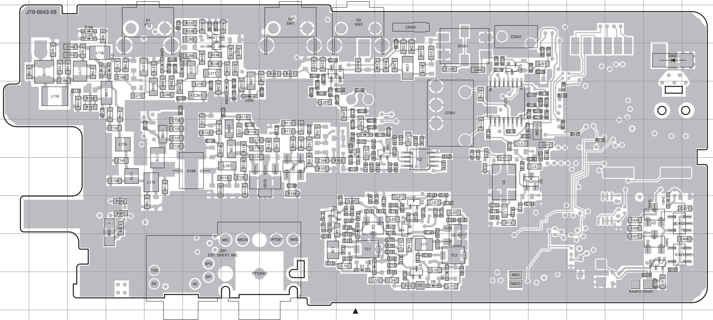
TX-RX UNIT (X57-6870-20) Foil side view (J79-0043-09)
