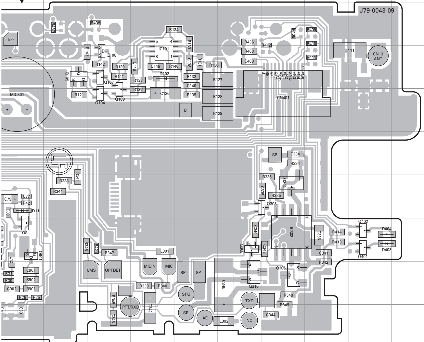
TX-RX UNIT (X57-6870-20) Component side view (J79-0043-09)
