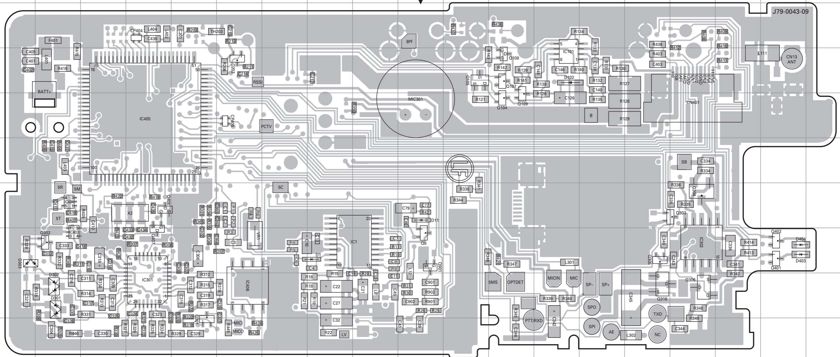
TX-RX UNIT (X57-6870-20) Component side view (J79-0043-09)
