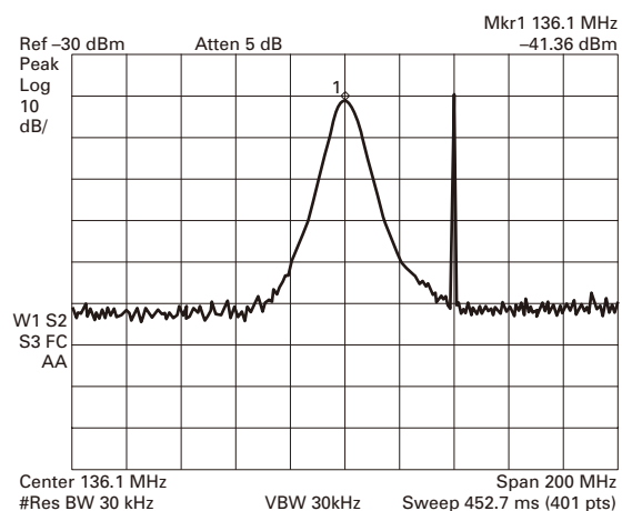
Fig. 3 Low-edge frequency
