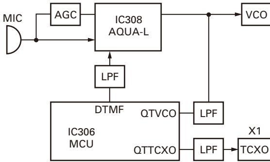
Fig. 6 Microphone amplifier
