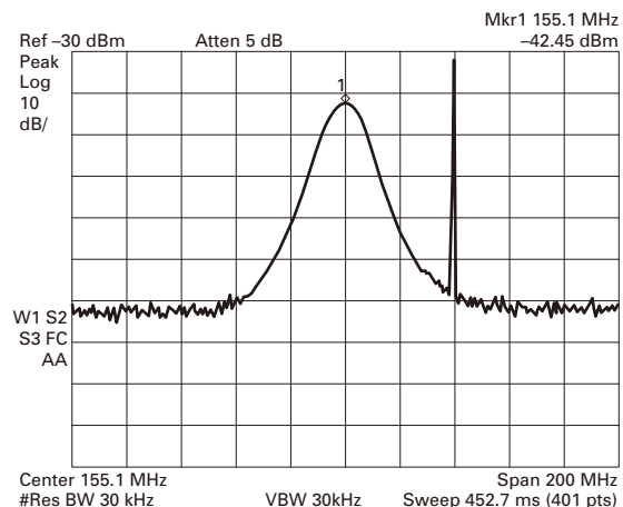
Fig. 1 Center frequency
