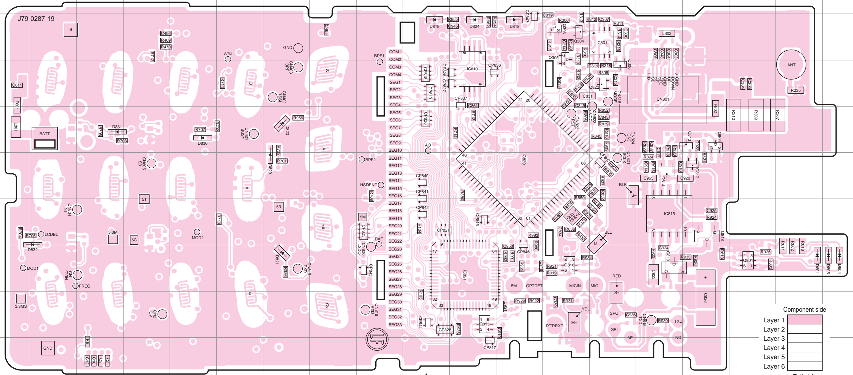
TX-RX UNIT (X57-7880-20) Component side view (J79-0287-19)
