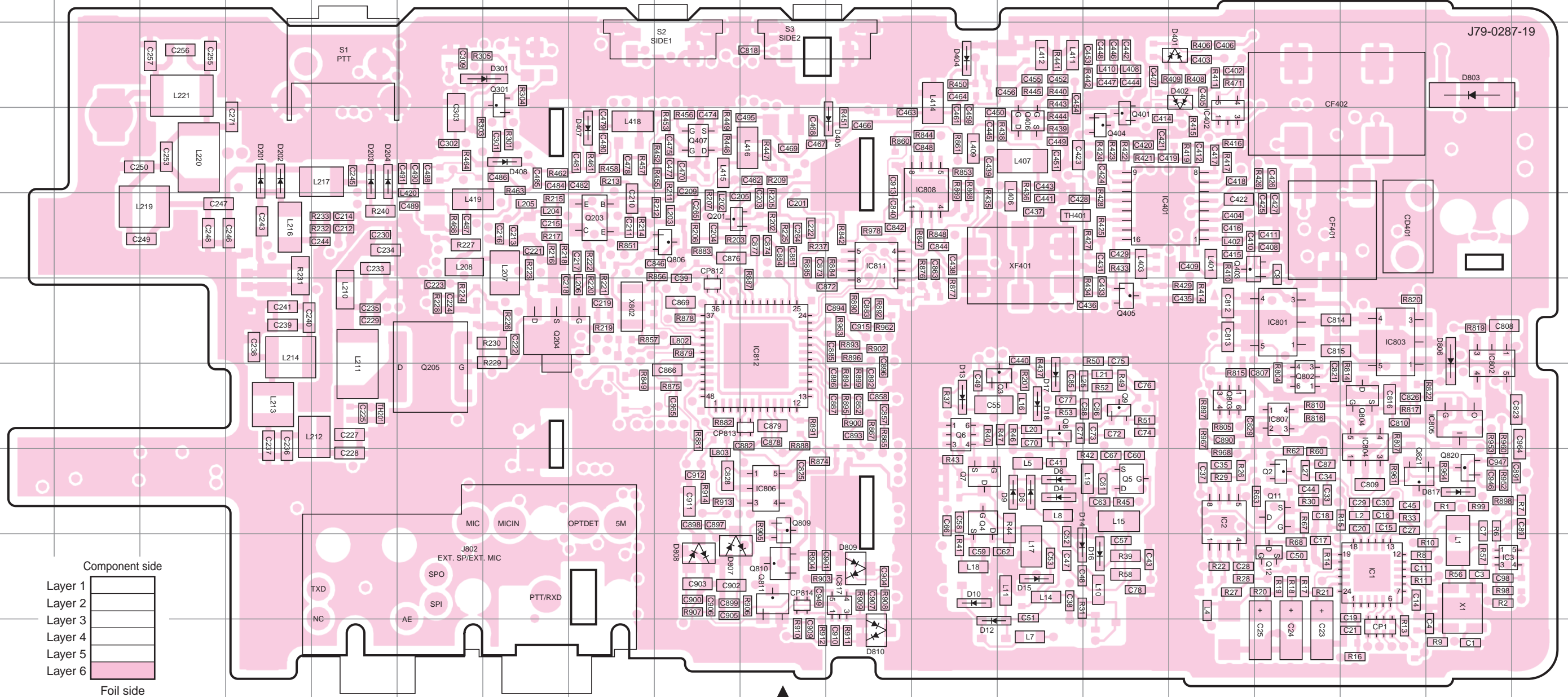
TX-RX UNIT (X57-7880-20) Foil side view (J79-0287-19)
