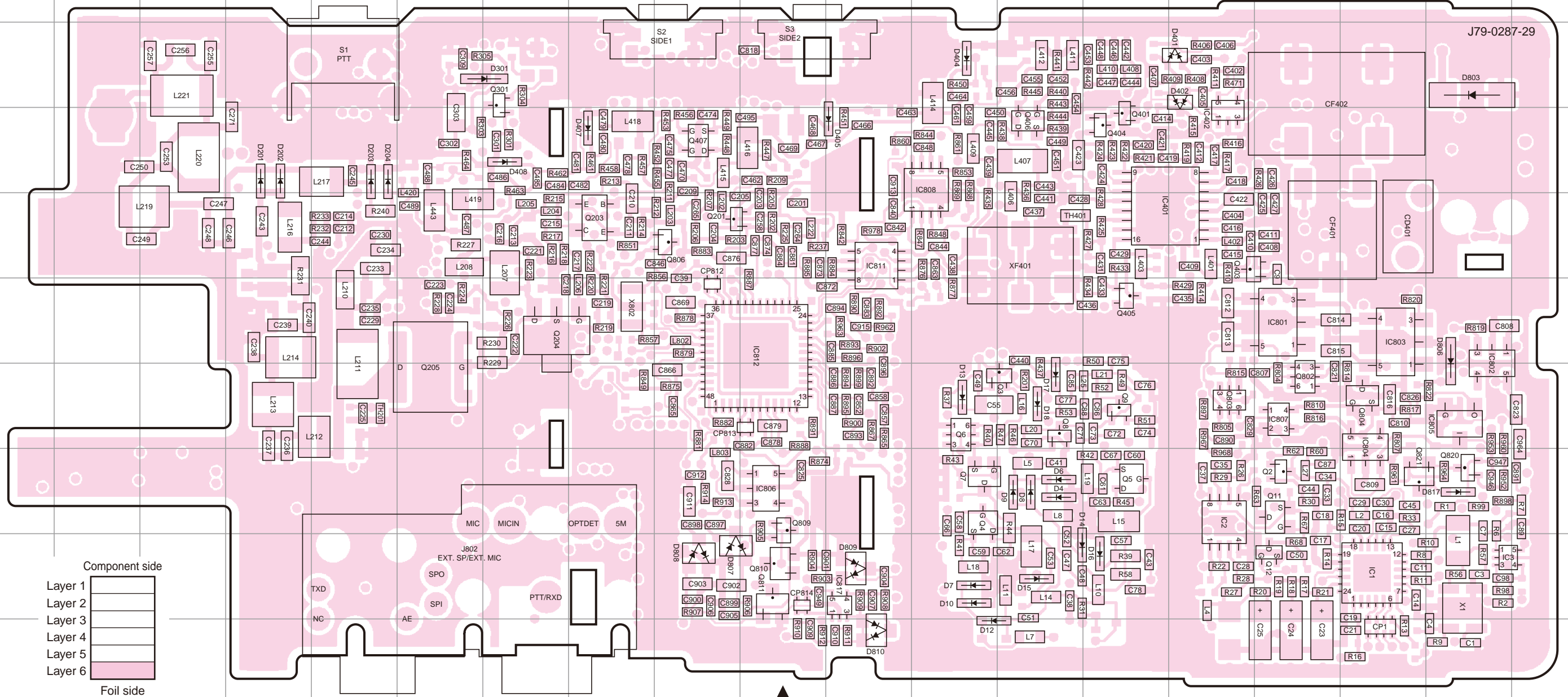
TX-RX UNIT (X57-7880-21) Foil side view (J79-0287-29)
