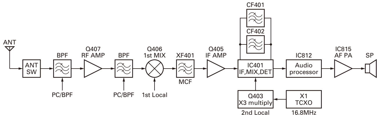
Fig. 2 Receiver system
