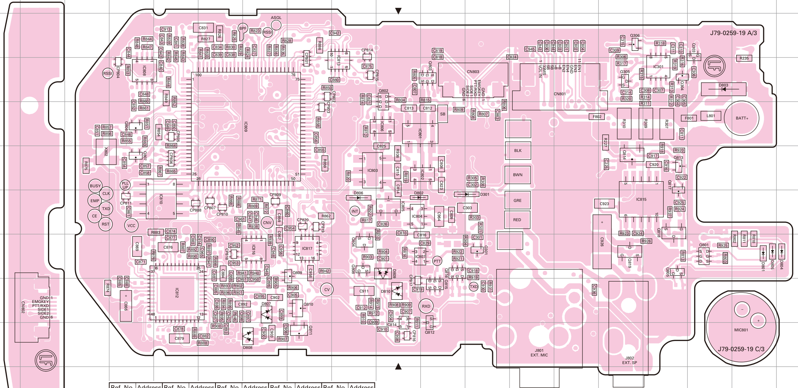
TX-RX UNIT (X57-7782-71) Component side view (J79-0259-19)
