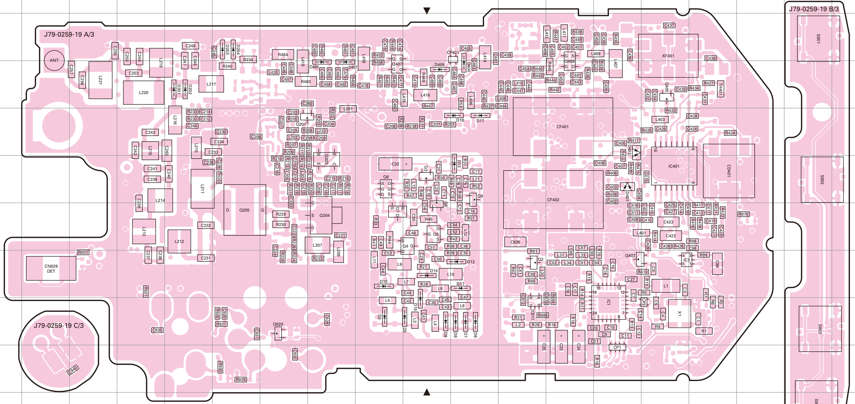
TX-RX UNIT (X57-7782-71) Foil side view (J79-0259-19)
