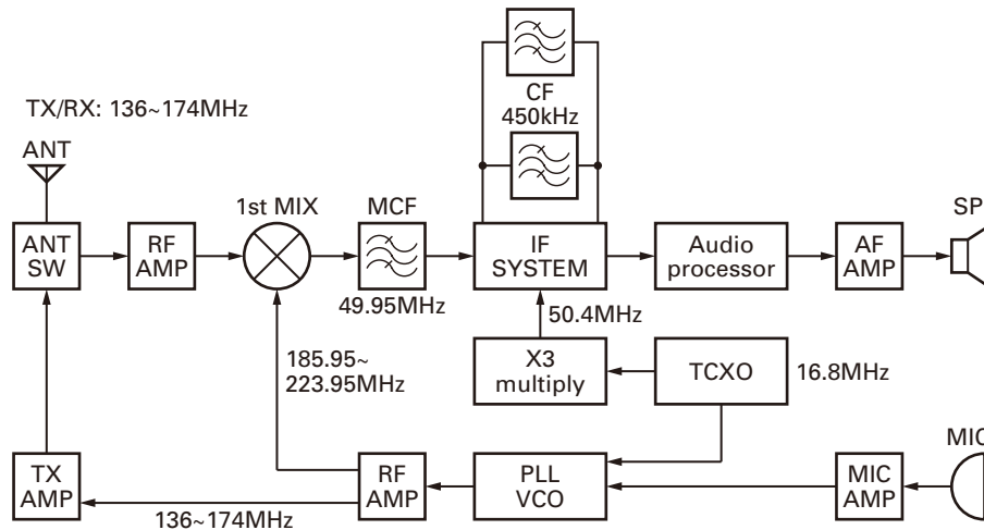
Fig. 1 Frequency configuration
