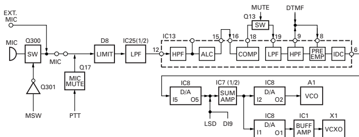
Fig. 7 Microphone amplifier
