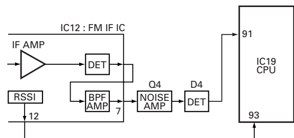
Fig. 5 Squelch circuit
