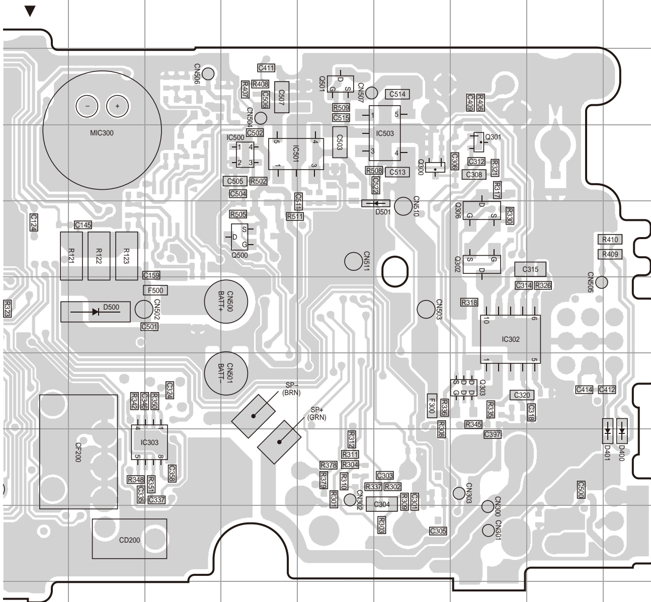
TX-RX UNIT (X57-8100-23) Component side view (J79-0306-19)
