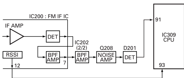
Fig. 5 Squelch circuit
