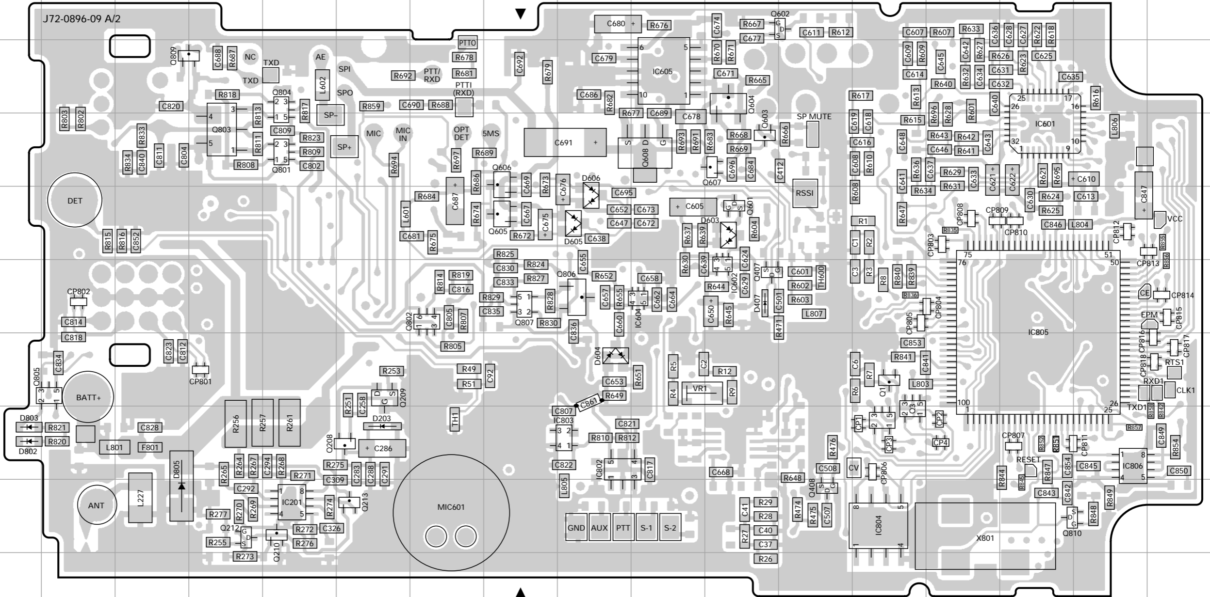
TX-RX UNIT (X57-6730-XX) -31 : A -32 : A3 Component side view (J72-0896-09)
