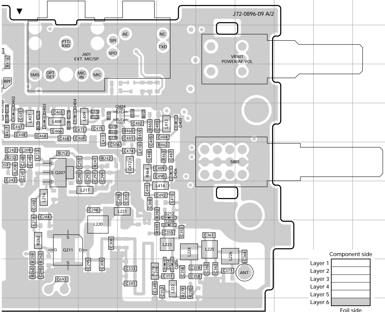
TX-RX UNIT (X57-6730-XX)
