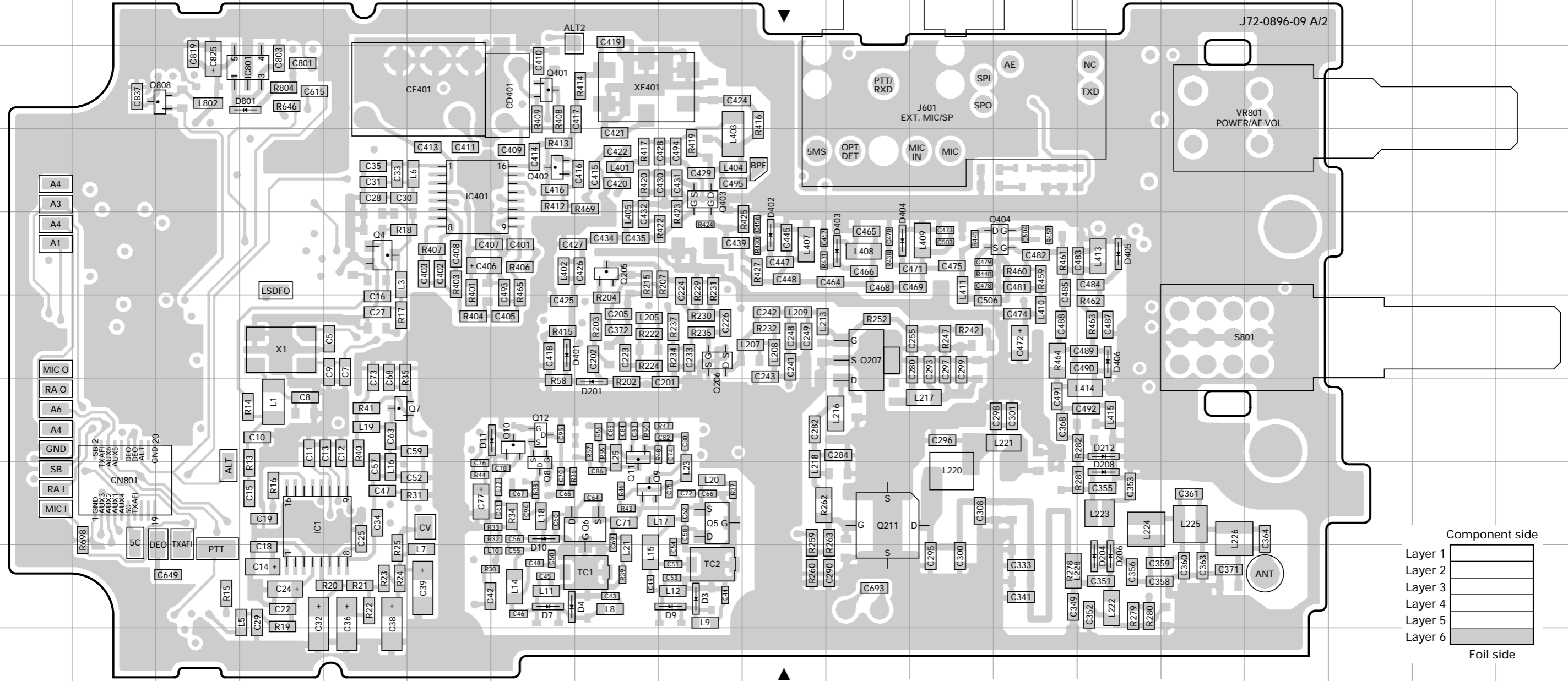
TX-RX UNIT (X57-6730-XX)
