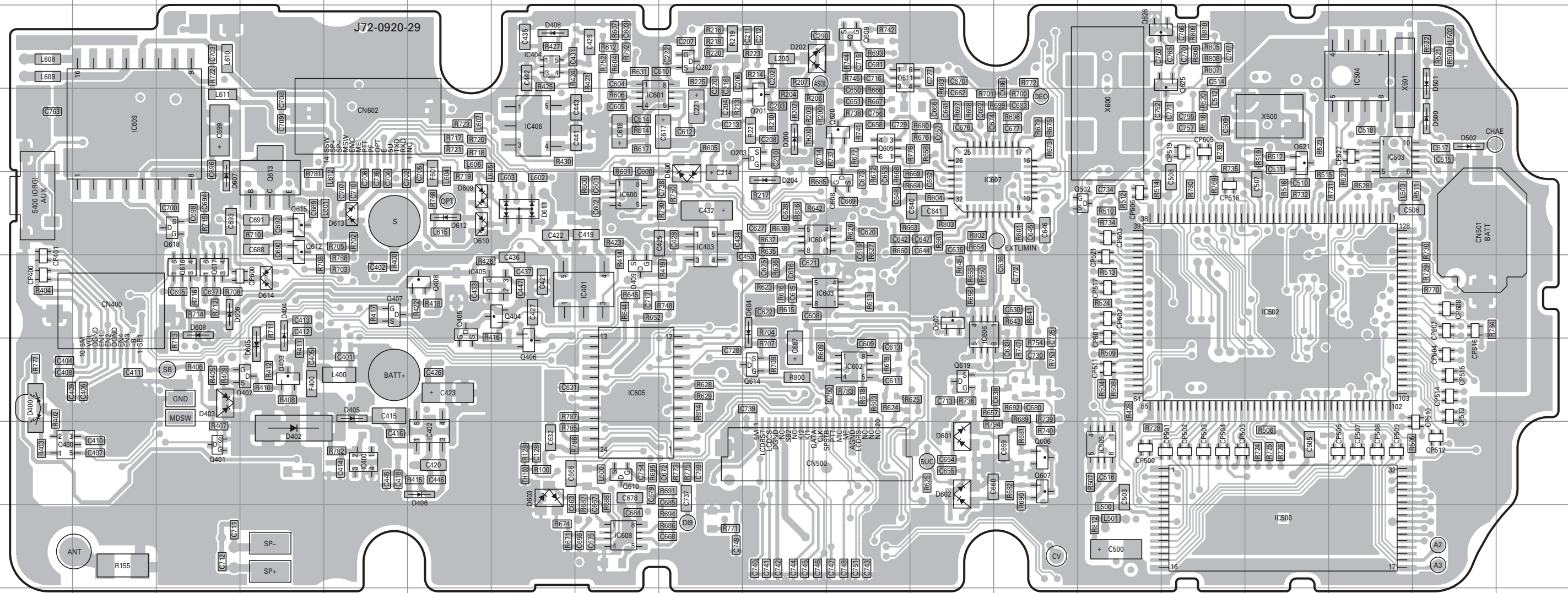
TX-RX UNIT (X57-6942-71) Component side view (J72-0920-29)
