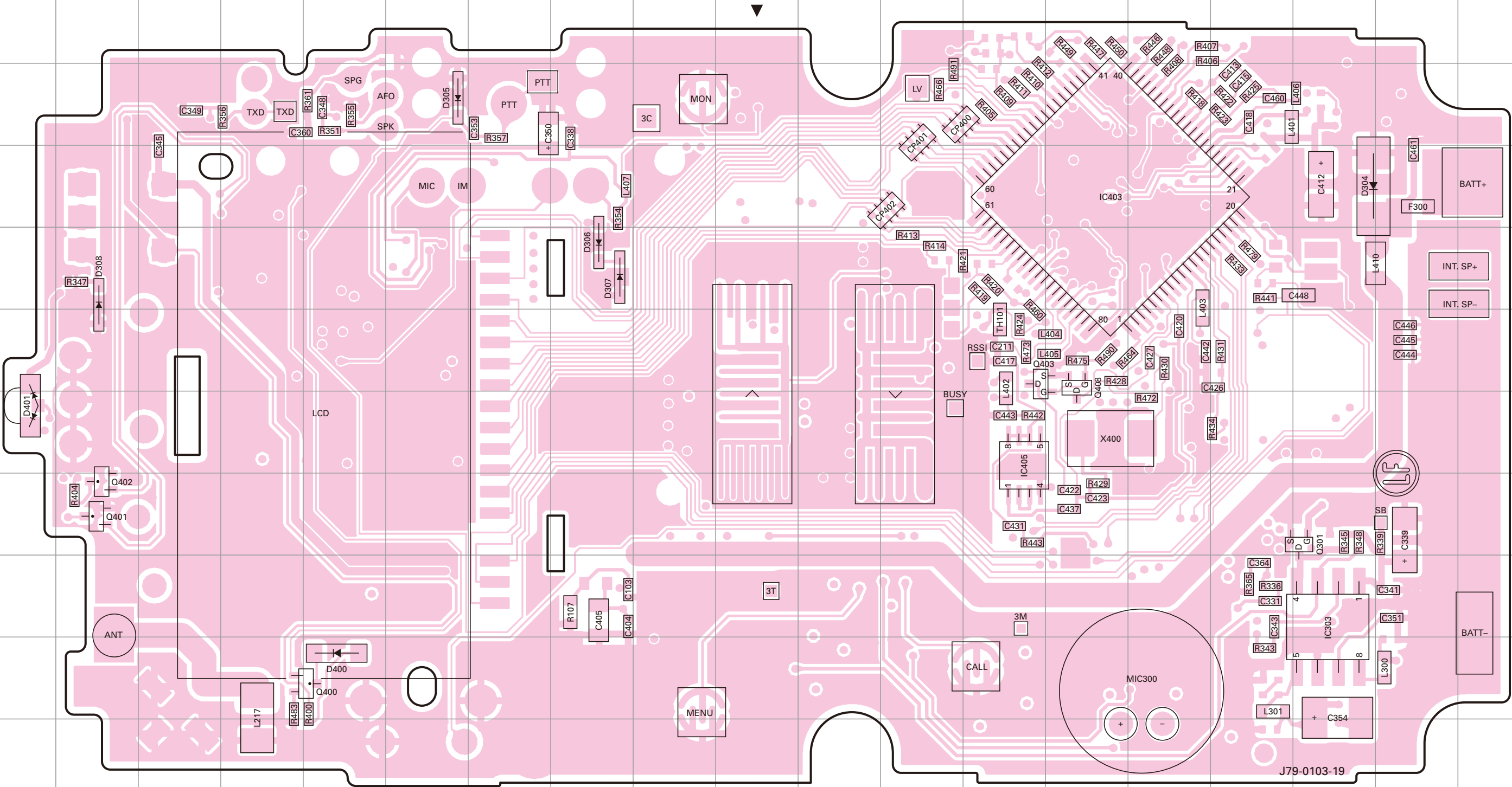
TX-RX UNIT (X57-7330-10) Foil side view (J79-0103-19)
