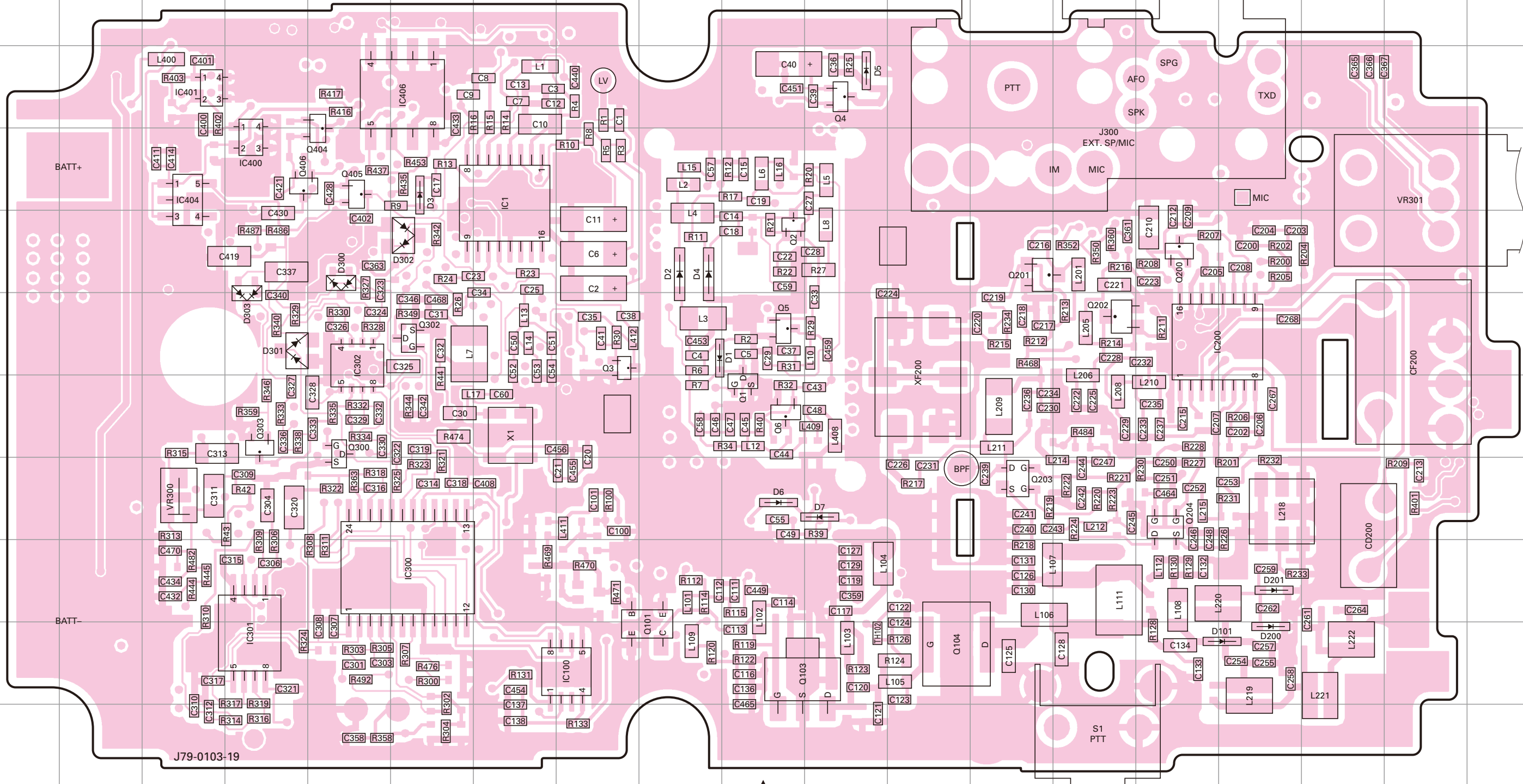
TX-RX UNIT (X57-7330-10) Component side view (J79-0103-19)
