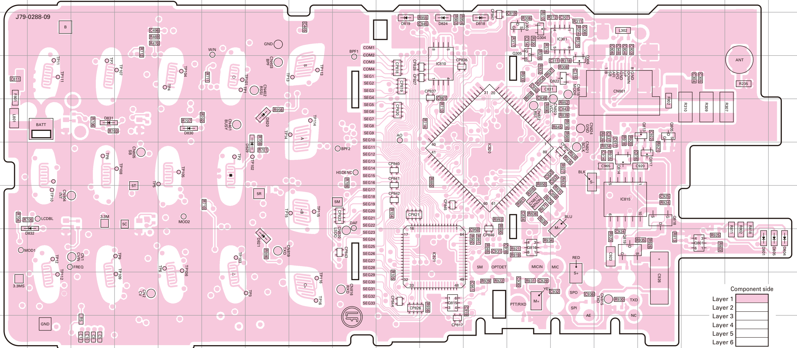
TX-RX UNIT (X57-7890-20) Component side view (J79-0288-09)
