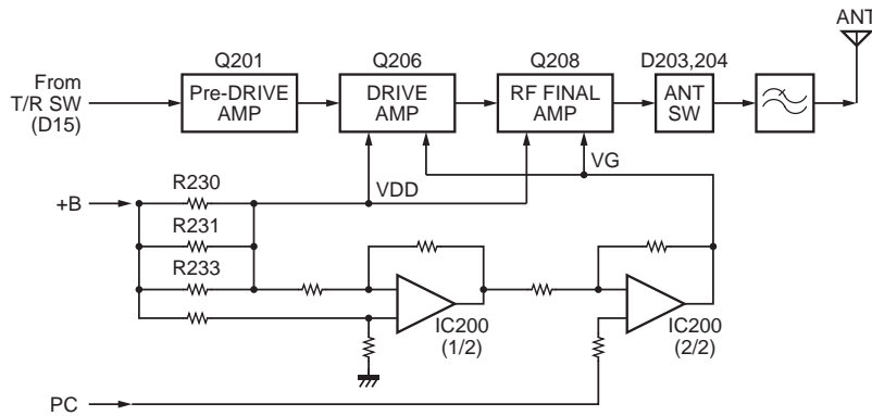
Fig. 5 Drive and final amplifier and APC circuit
