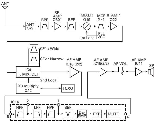
Fig. 2 Receiver section
