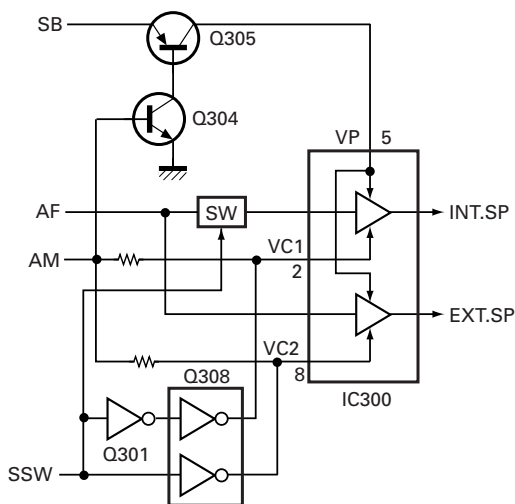
Fig. 3 Audio amplifier circuit
