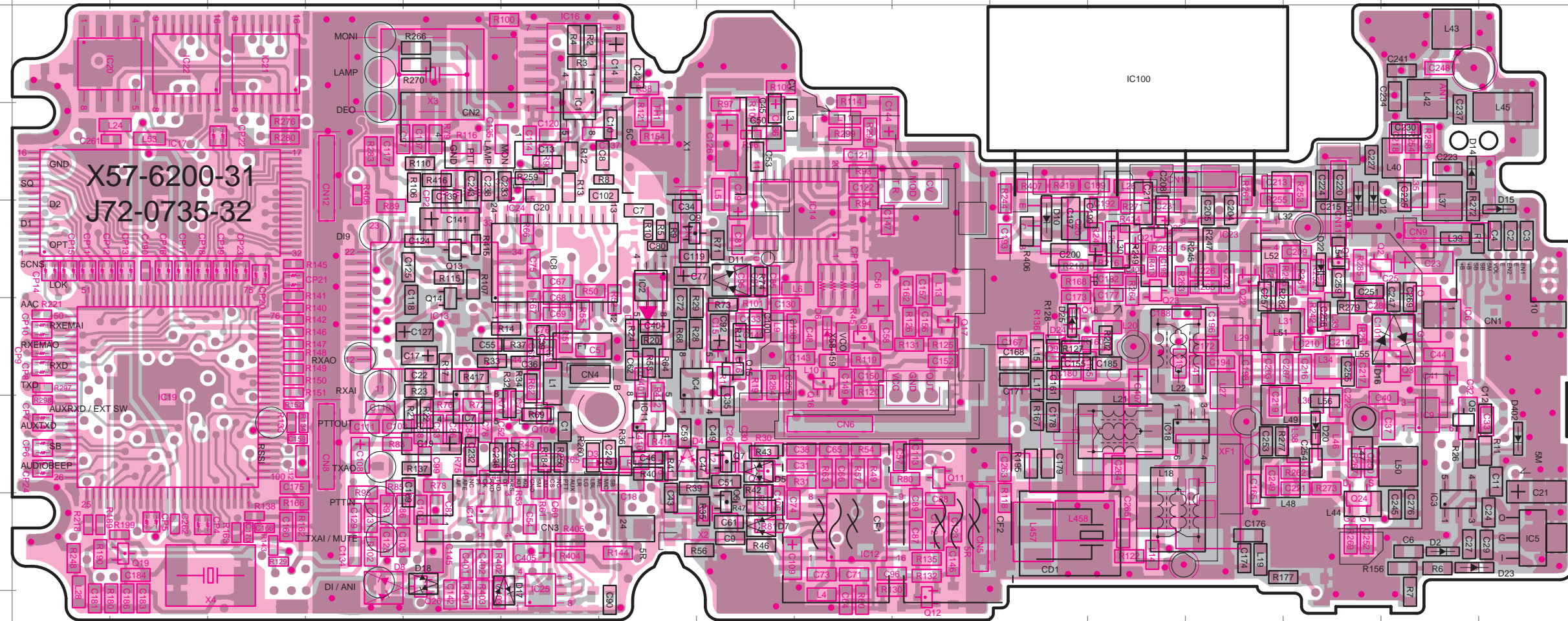
TX-RX UNIT (X57-6200-31) Component Side + Foil Side View
