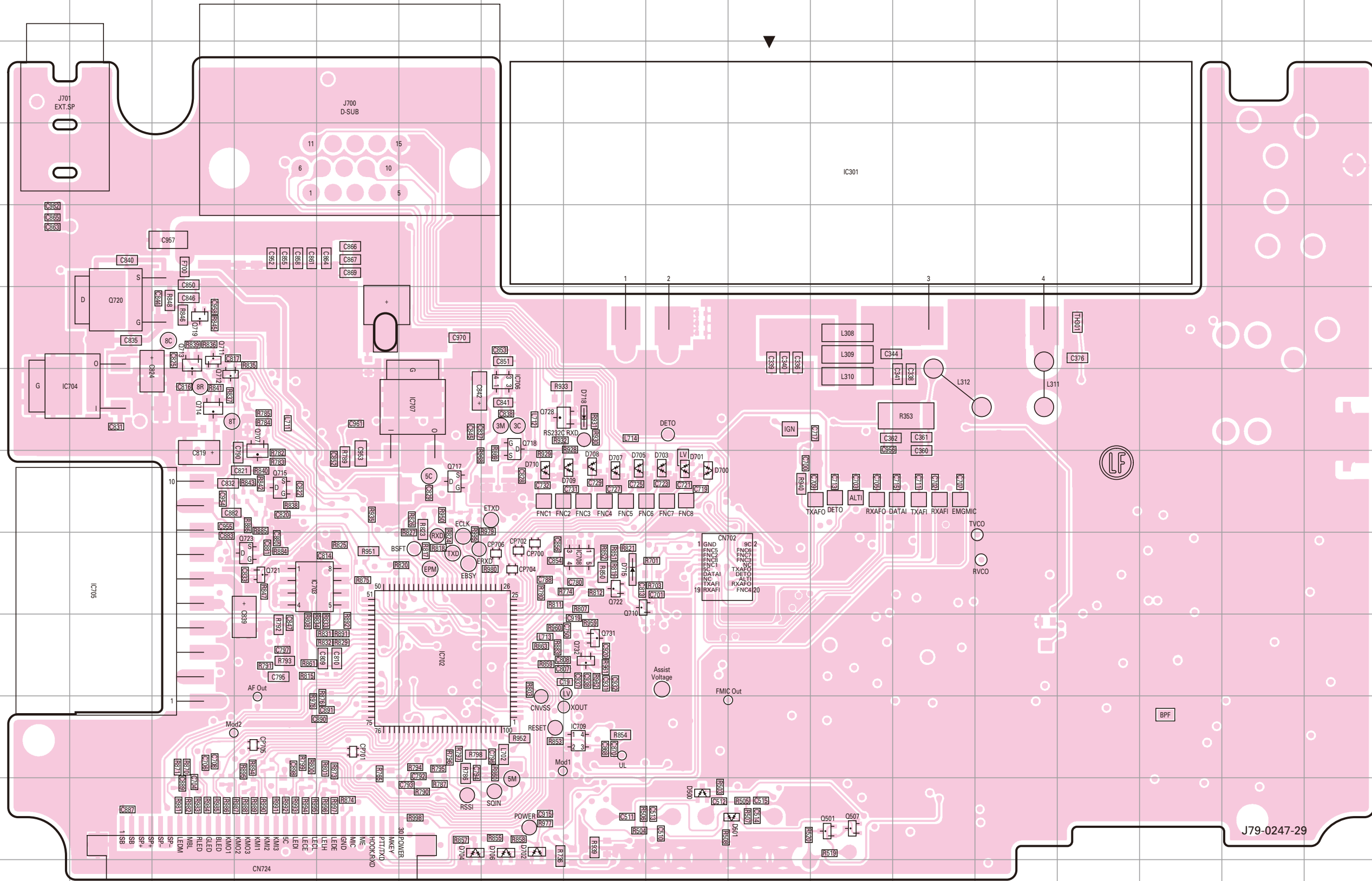
TX-RX UNIT (X57-7683-01) Component side view (J79-0247-29)
