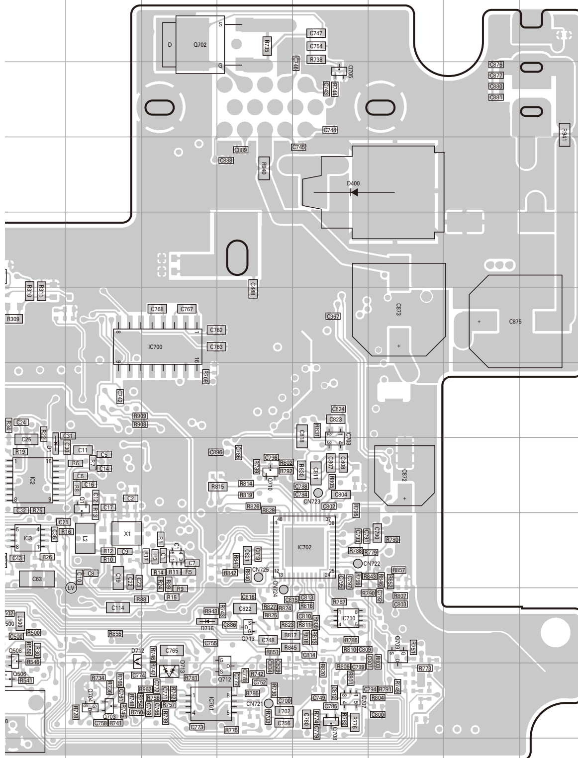
TX-RX UNIT (X57-8020-21) Foil side view (J79-0296-09)
