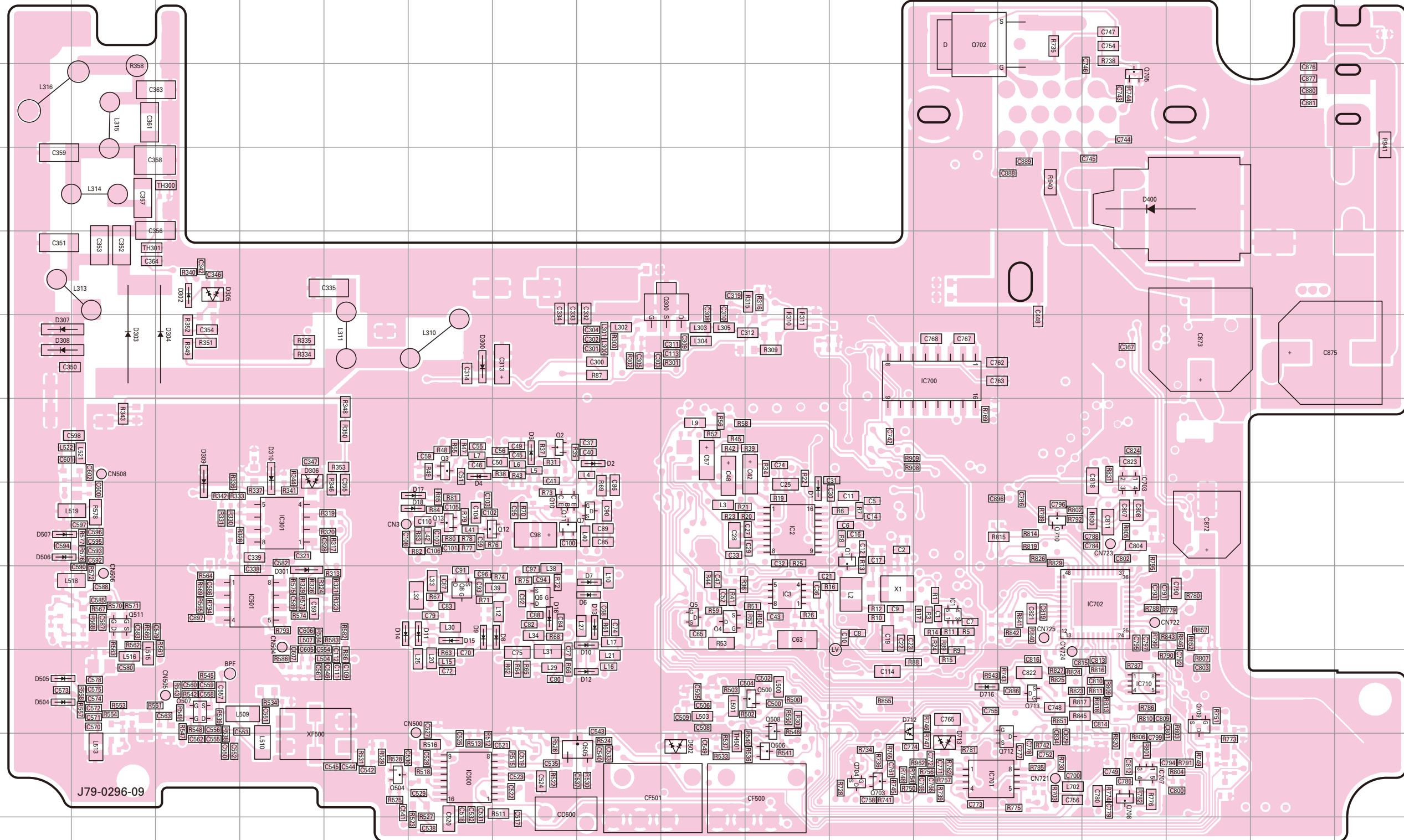
TX-RX UNIT (X57-8020-21) Foil side view (J79-0296-09)
