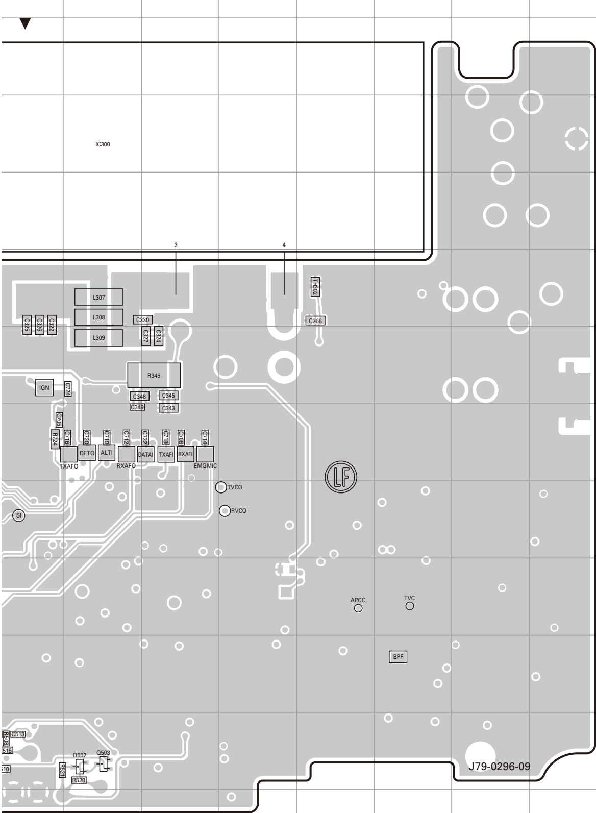
TX-RX UNIT (X57-8020-21) Component side view (J79-0296-09)
