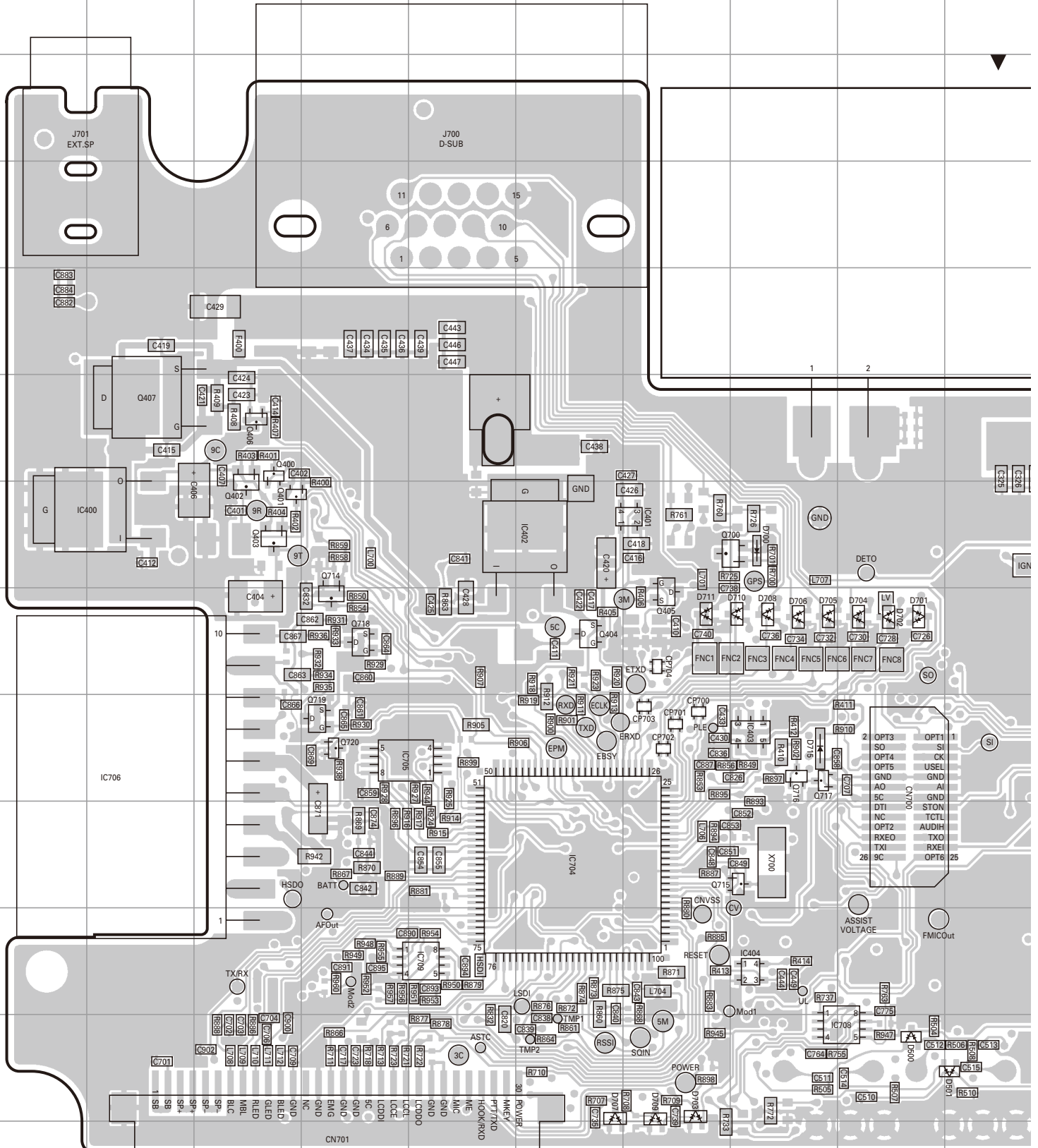
TX-RX UNIT (X57-8020-21) Component side view (J79-0296-09)
