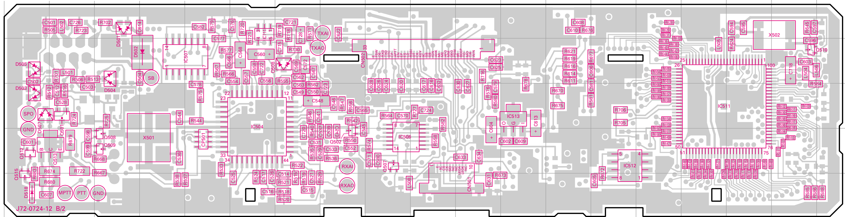
TX-RX UNIT (X57-6142-70) (B/2) Foil side view
