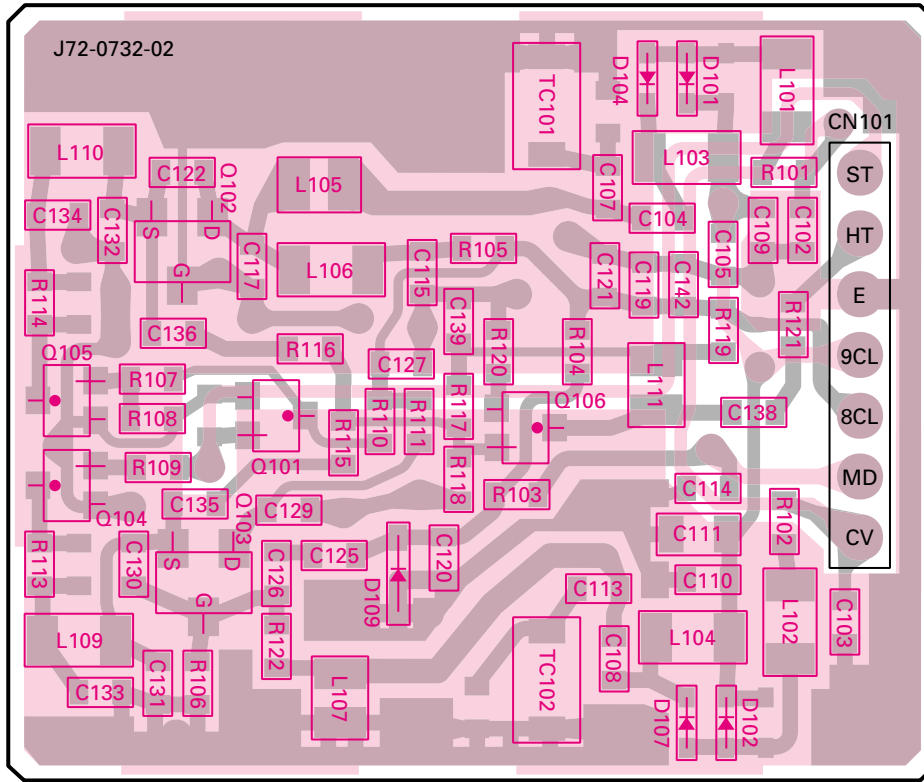
PLL/VCO (X58-4712-70) Component side view
