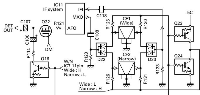
Fig. 3 Wide/Narrow changerover circuit
