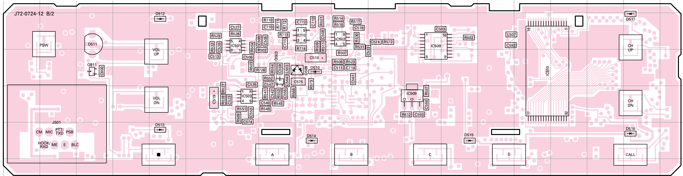
TX-RX UNIT (X57-6142-70) (B/2) Component side view
