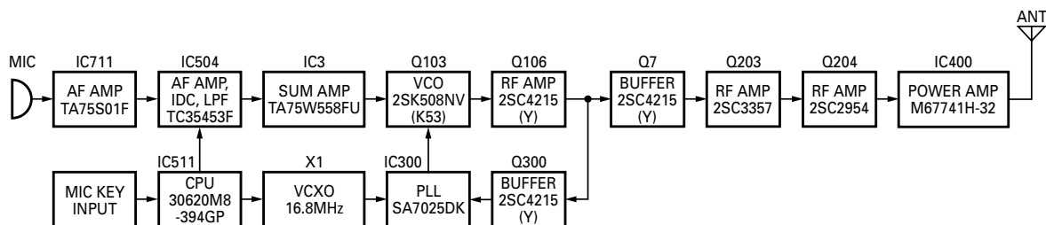
Fig. 6 Transmitter system
