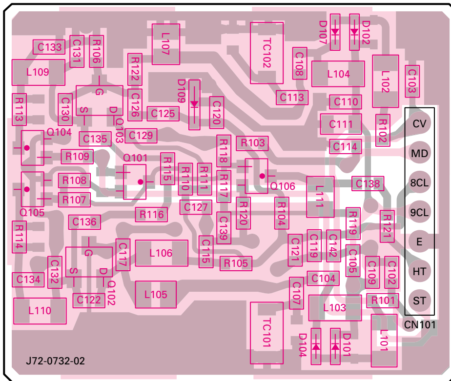
PLL/VCO (X58-4712-70) Foil side view
