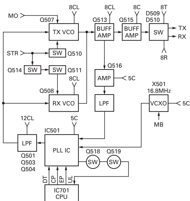
Fig. 4 PLL circuit
