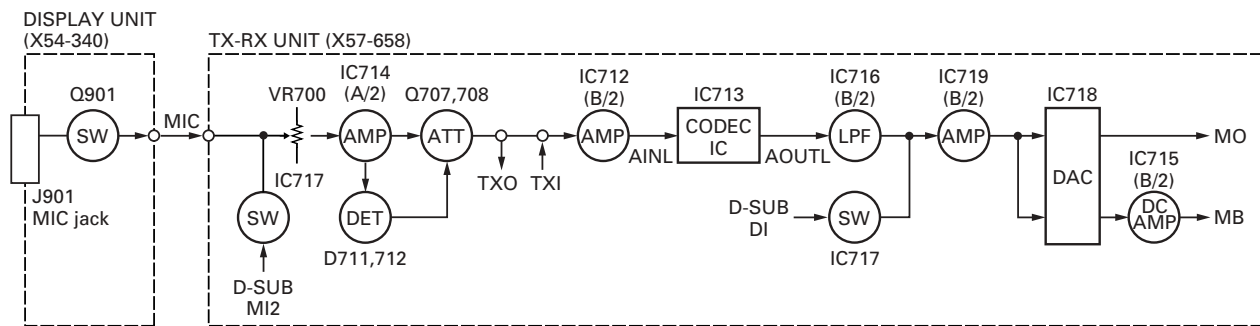
Fig. 2 Microphone circuit
