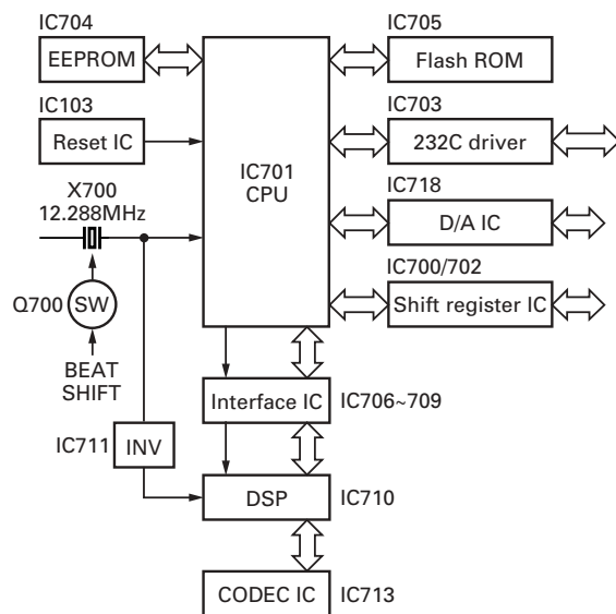
Fig. 5 Control circuit
