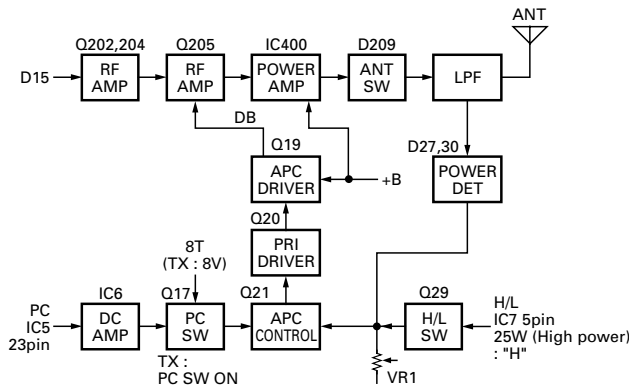
Fig. 7 APC circuit
