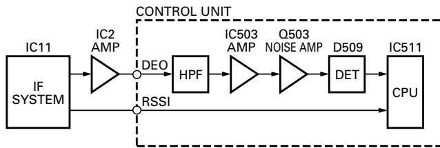
Fig. 4 Squelch circuit
