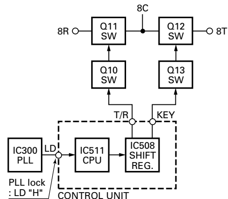
Fig. 6 Unlock circuit
