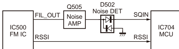
Fig. 5 Squelch circuit
