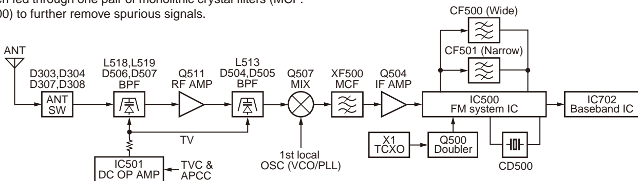
Fig. 2 Receiver System
