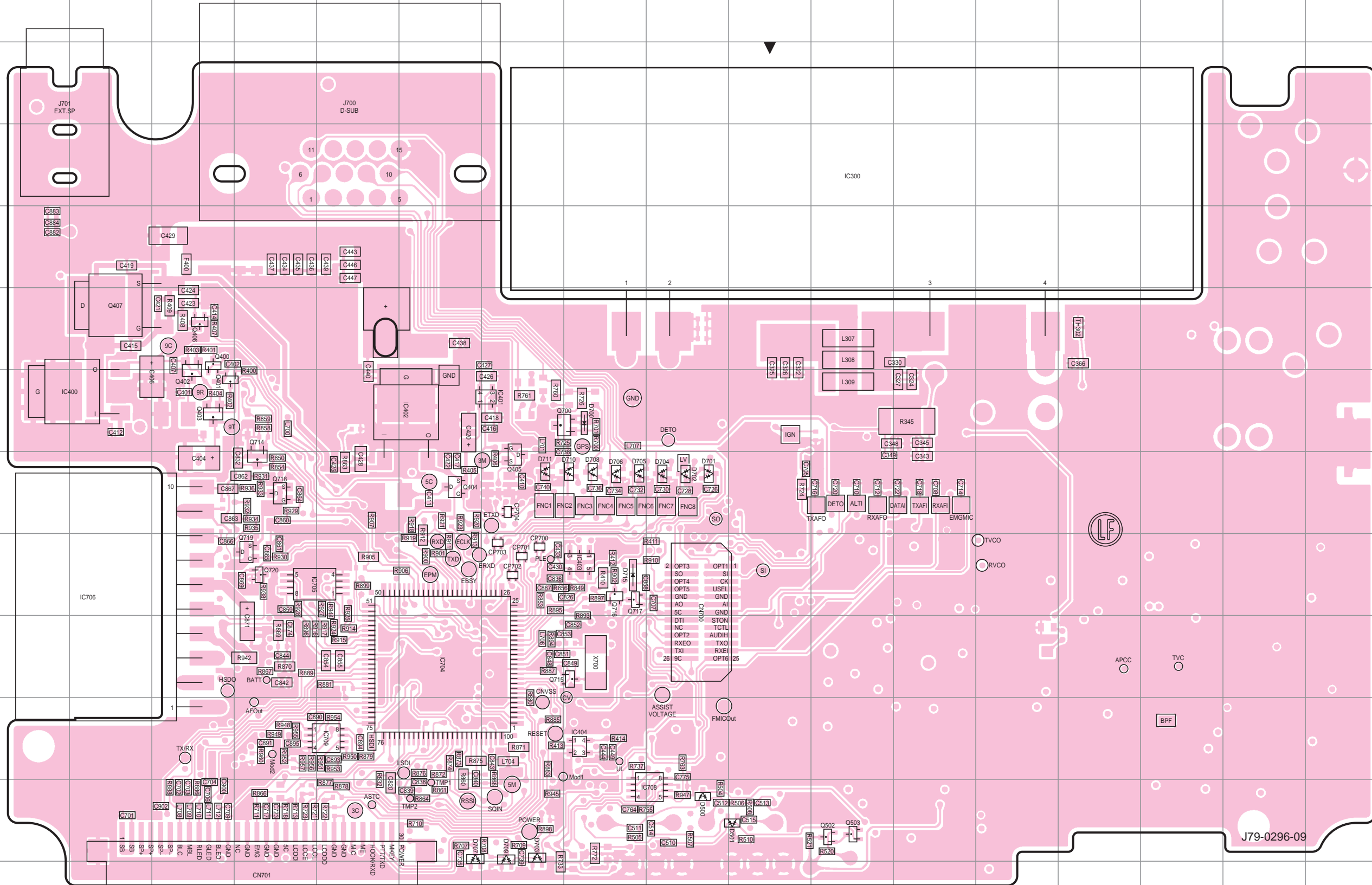
TX-RX UNIT (X57-8020-21) Component side view (J79-0296-09)
