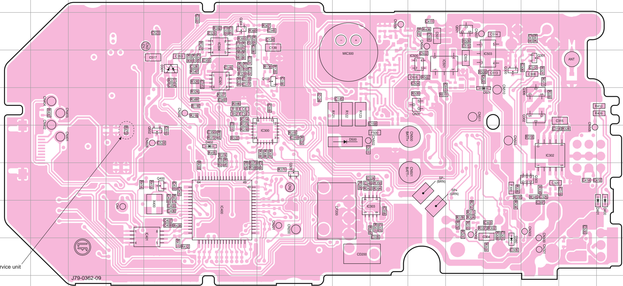
TX-RX UNIT (X57-8093-00) Component side view (J79-0362-09)
