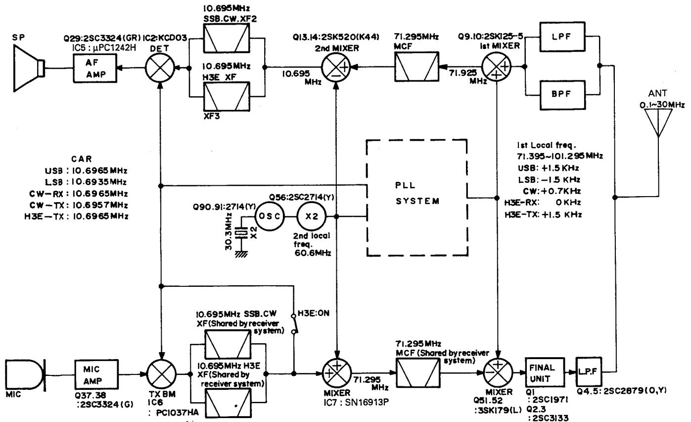
Fig. 1 Frequency configuration
