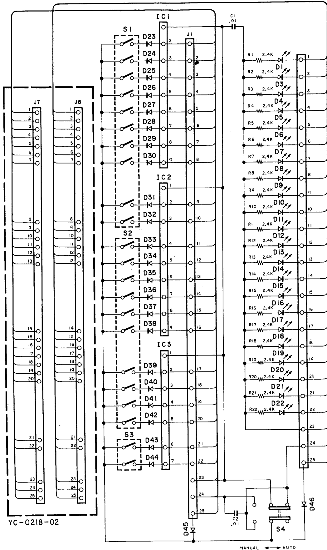
Fig. 12 LED unit
