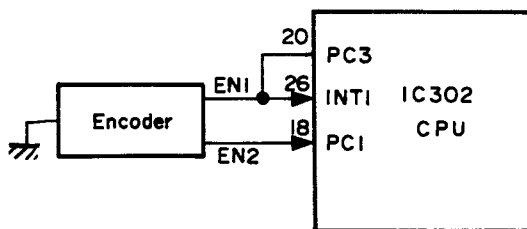
Fig. 11 Encoder circuit
