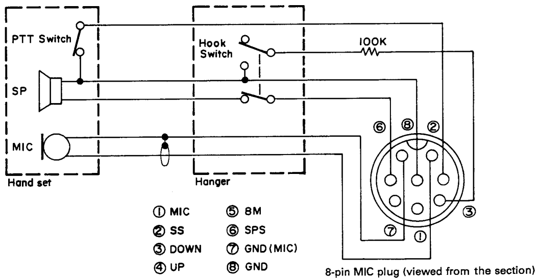
Fig. 22 Handset connection
