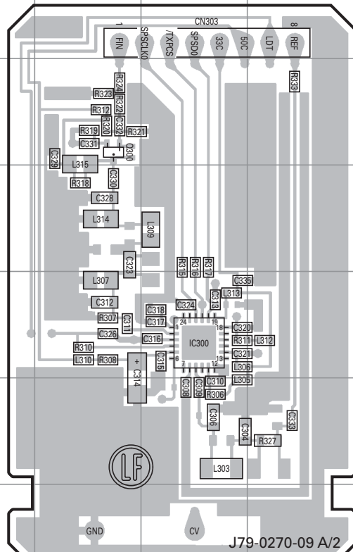
TX VCO/PLL UNIT (X58-5220-10) Foil side view (J79-0270-09)
