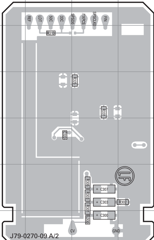
TX VCO/PLL UNIT (X58-5220-10) Component side view (J79-0270-09)
