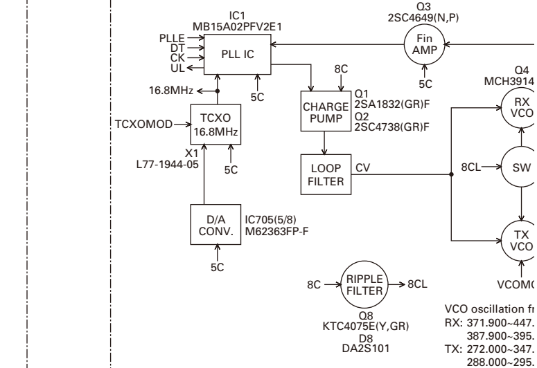
TX-RX UNIT (X57-8130-XX A/2): TX-RX section
