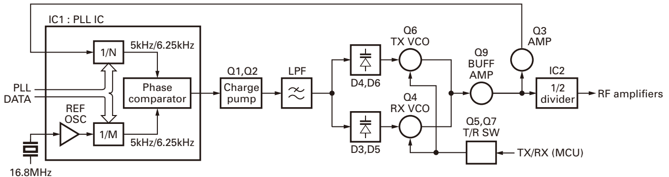
Fig. 6 PLL circuit
