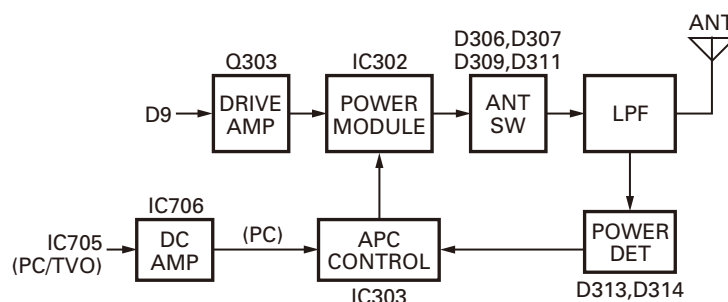
Fig. 9 APC circuit
