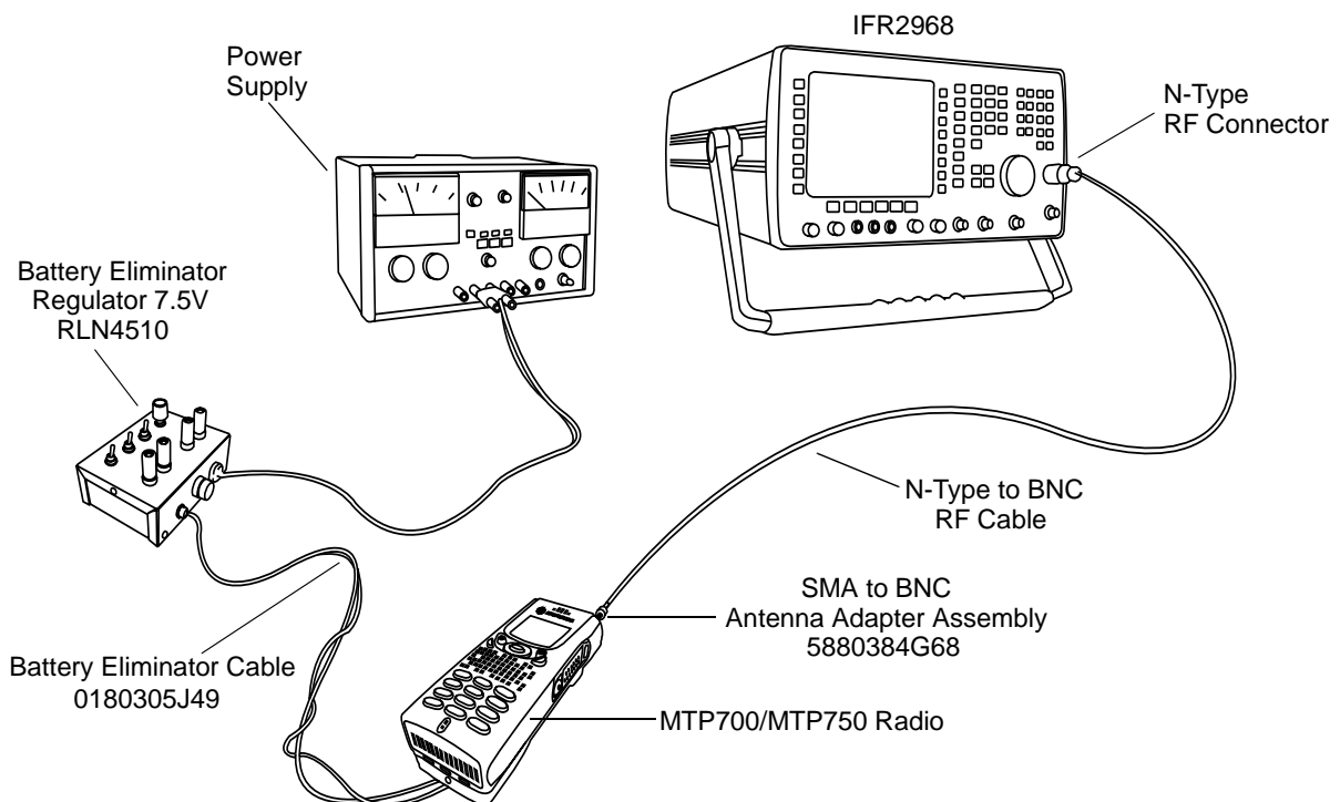
Figure 5-1 Typical Test Setup
