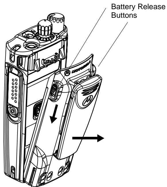
Figure 6-1 Battery Removal
