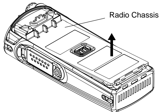
Figure 6-3 Chassis Removal
