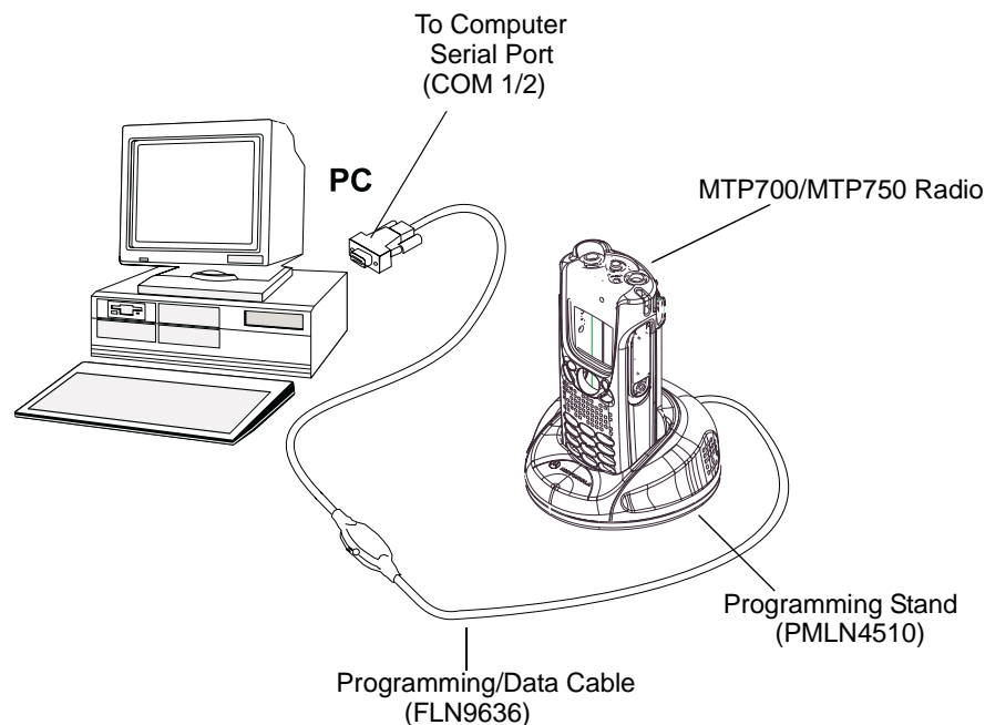
Figure 4-1 Setup for Radio Programming.
