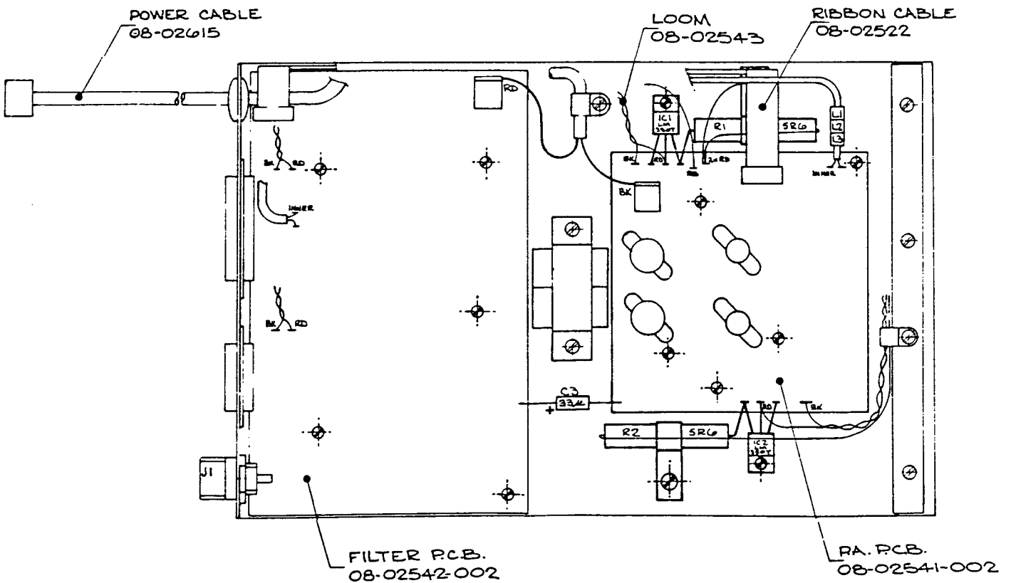
4402 24v.200w. P.A. CHASSIS COMPONENT LAYOUT.
