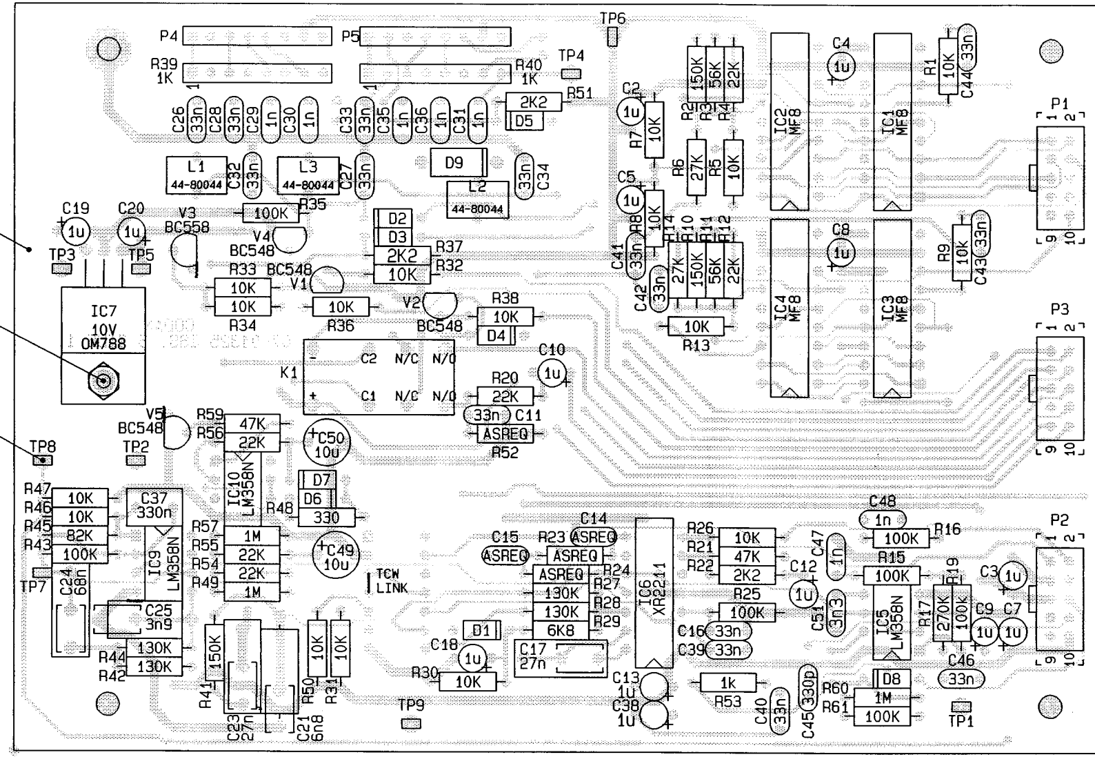
PCB 07-01325 ISSUE 3
