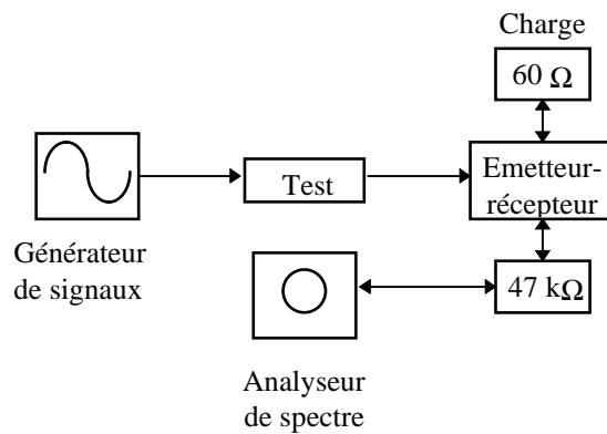
Figure 7-4: Configuration du test
