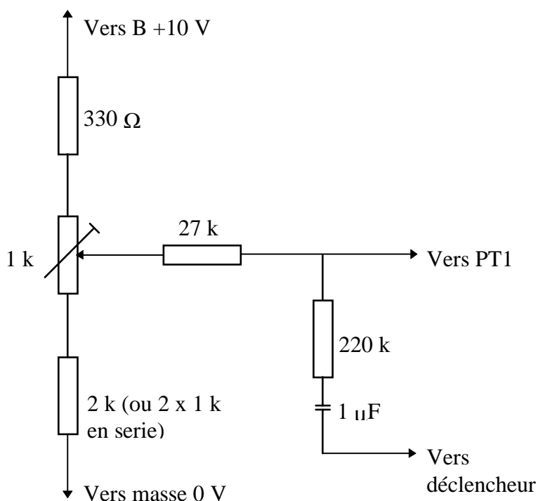
Figure 7-3: Circuit du kit d'essai
