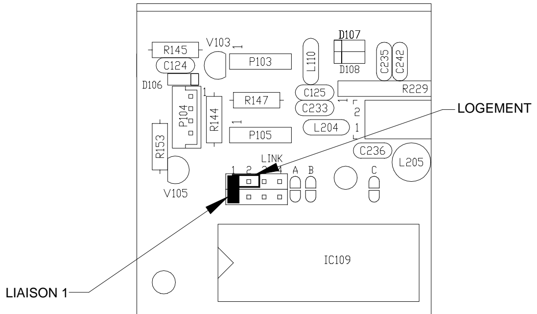
Figure 7-1: Position LINK 1
