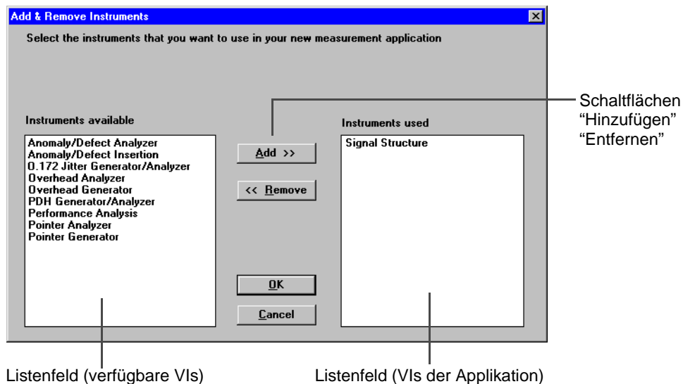
Bild B-15 Dialogfenster "Add & Remove Instruments" des Application Managers
