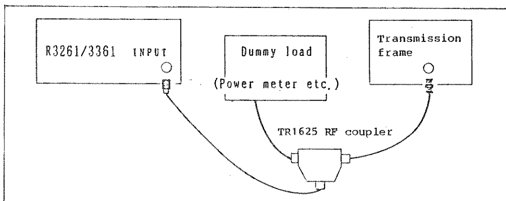
Figure 6 - 1 Measuring the Deviation of the Signal
