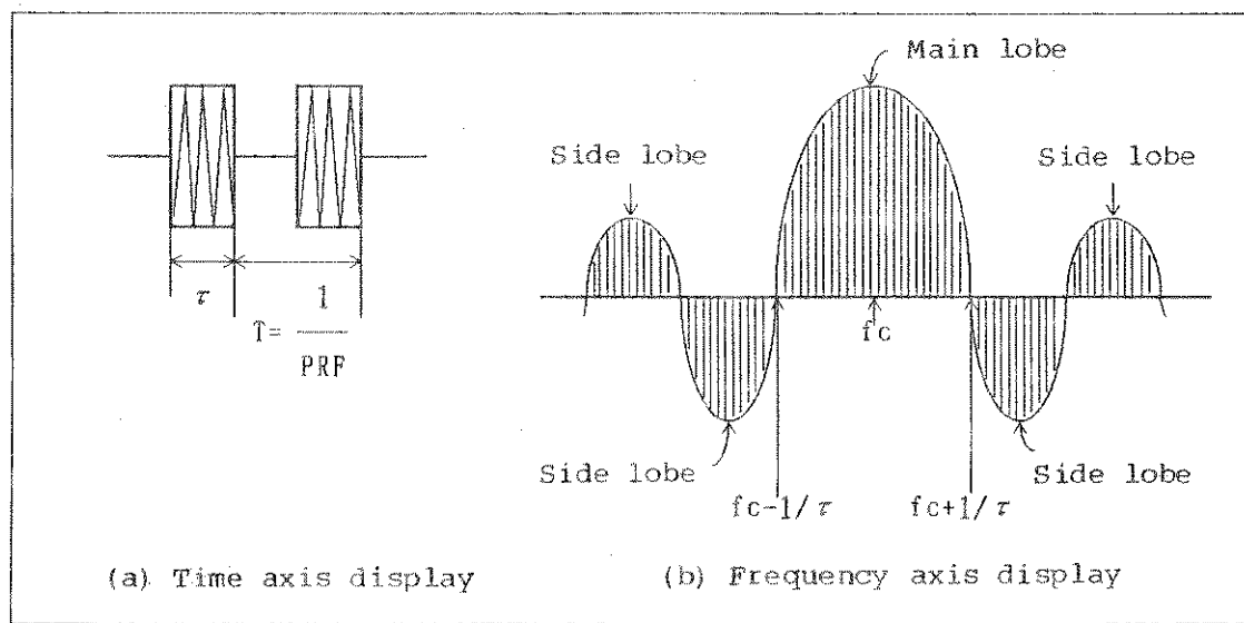
Figure 6 - 7 Pulse Modulation Wave
