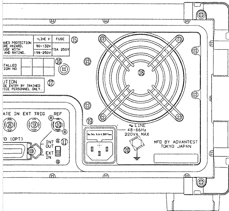
Figure 2 - 2 Rear Panel
