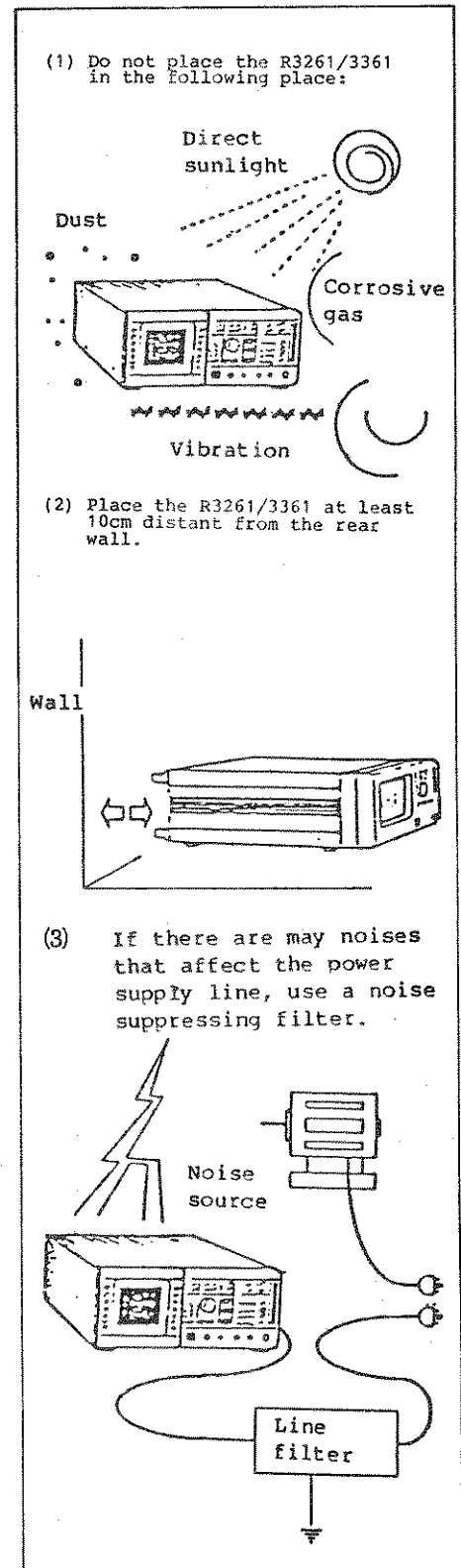
Figure 1 - 1 Environmental Conditions
