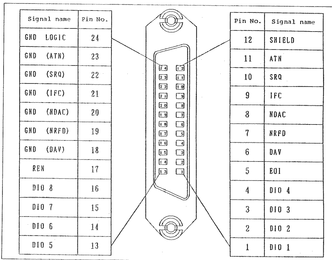
Figure 7 - 2 GPIB Connector Pin Configuration
