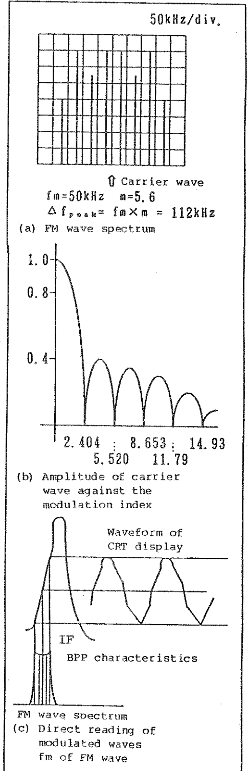
Figure 6 - 4 FM Signal
