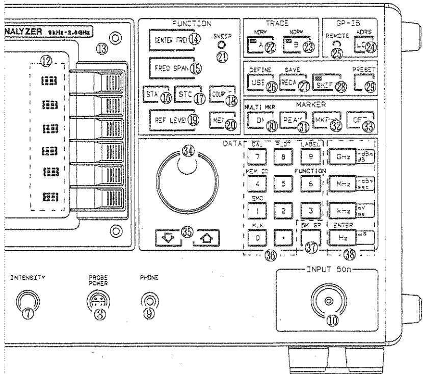
Figure 2 - 1 Front Panel
