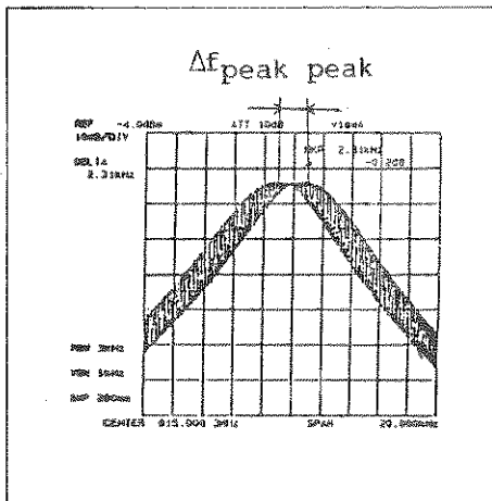
Figure 6 - 5 When \Delta f_{\text{peak}} is small
