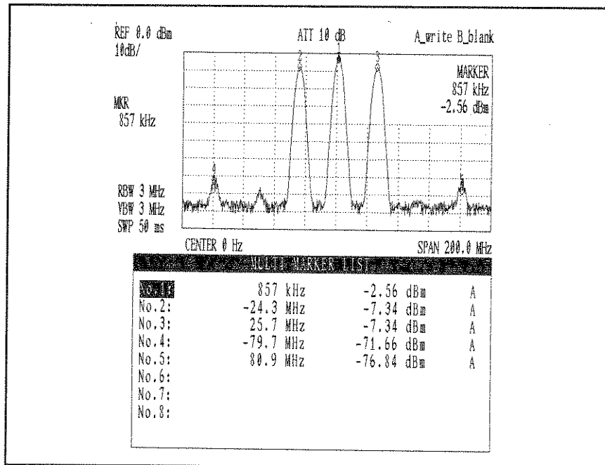
Figure 5.15-4 Printing Precision Set at HIGH (Half Size)
