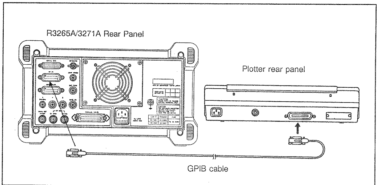
Figure 5.9-1 Plotter Connection
