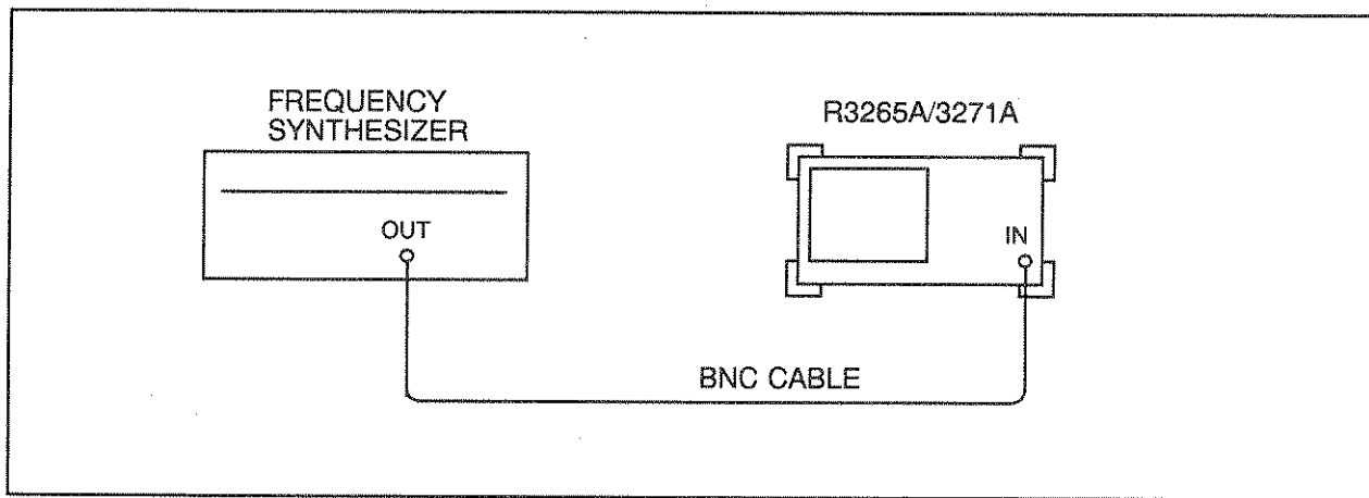
Figure 4-3 Residual FM Test Setup
