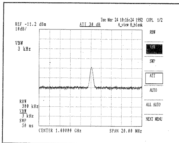
Figure 5.1-8 VBW = 3kHz
