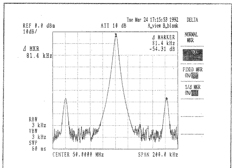
Figure 5.3-2 Delta Marker
