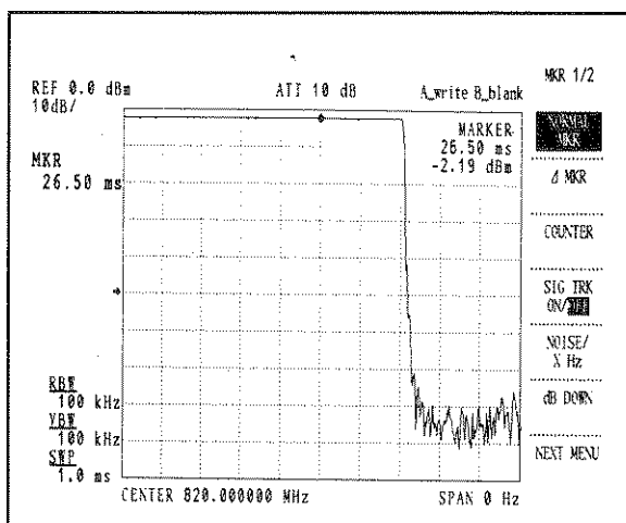
Figure 7 - 25 Full-Screen Display (DELAYED SWEEP ON)
