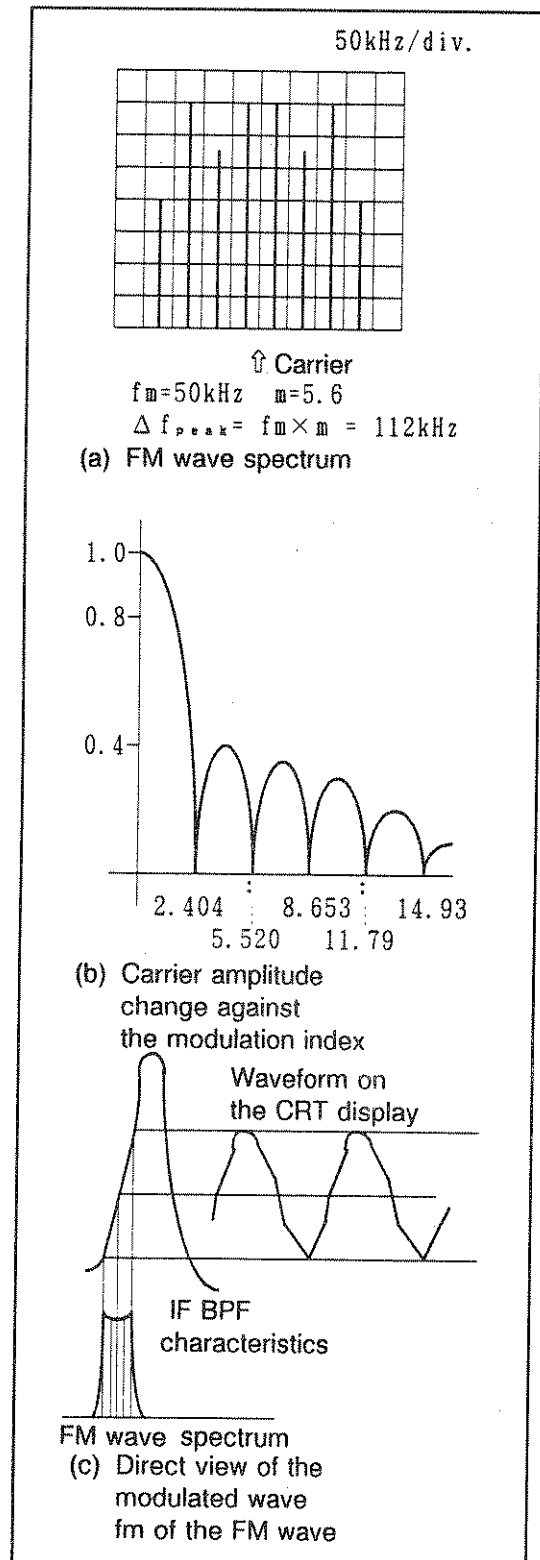
Figure 4-9 Measuring an FM Signal
