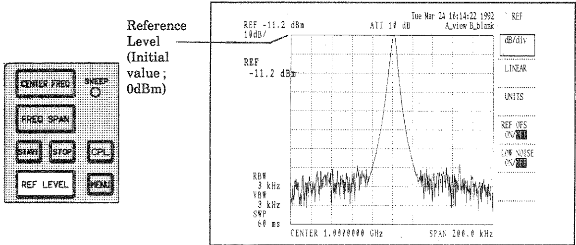
Figure 5.1-5 Reference Level
