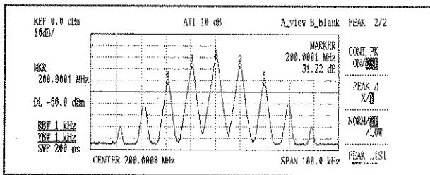
Figure 5.3-10 NEXT PK when UP is selected
