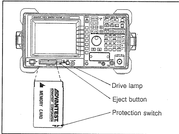
Figure 5.5-2 Inserting and Removing the Memory Card
