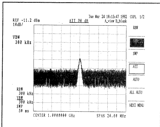
Figure 5.1-7 VBW = 300kHz
