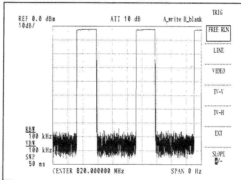
Figure 7 - 26 Full-Screen Display
