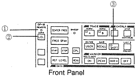
Front Panel
