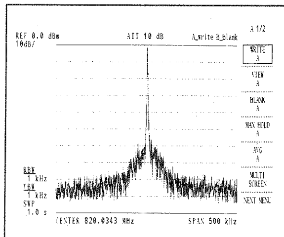
Figure 7 - 17 Full-Screen Display (GATED SWEEP ON)
