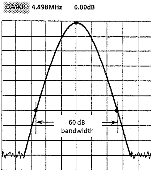
(b) 60 dB dropped bandwidth
