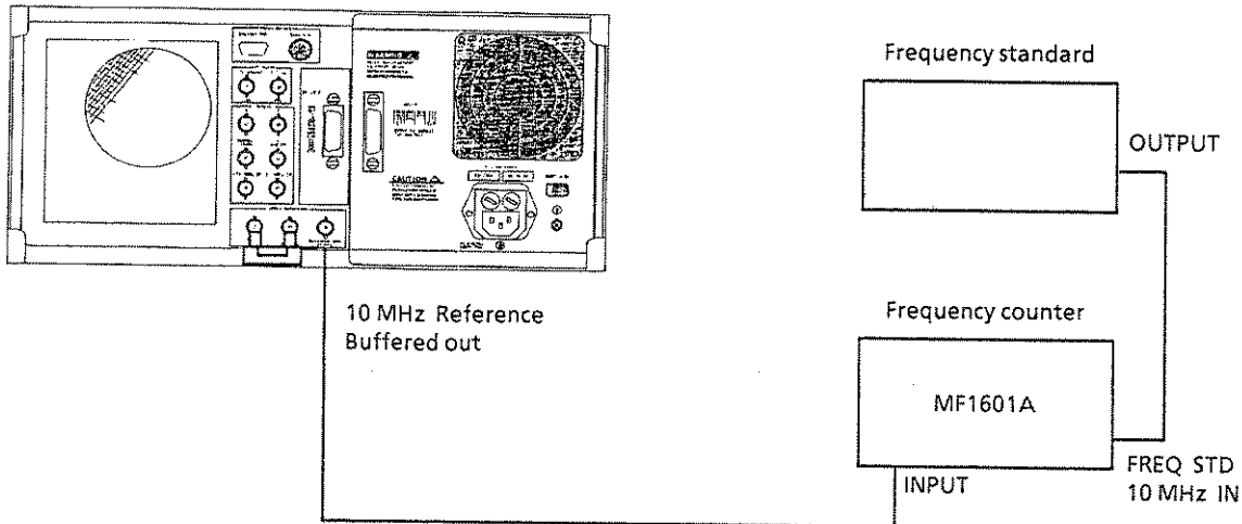
Reference Oscillator Frequency Stability Test
