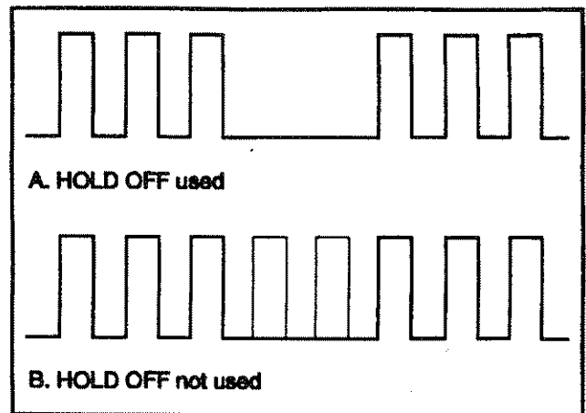
Fig. 5. Use of HOLDOFF Control
