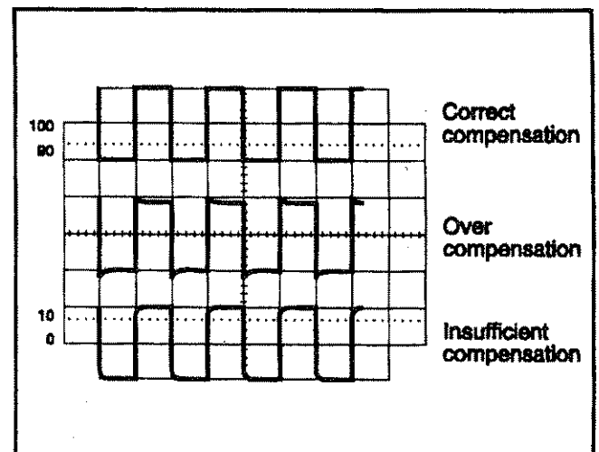
Fig. 6. Probe Compensation Adjustment
