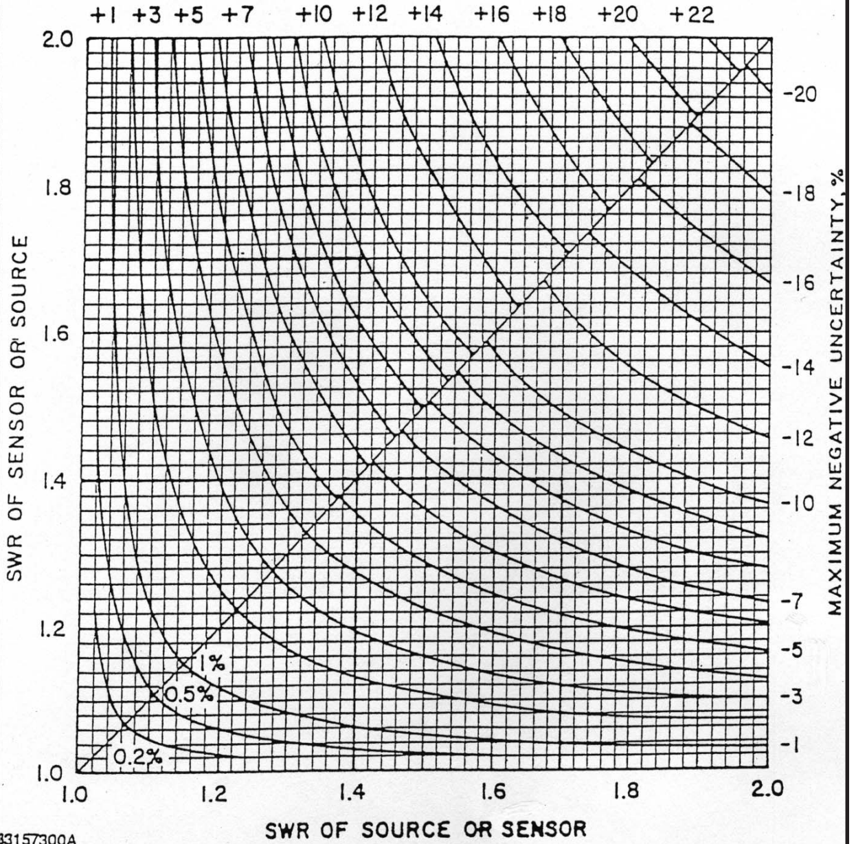
Figure 6-1. Mismatch Uncertainty
