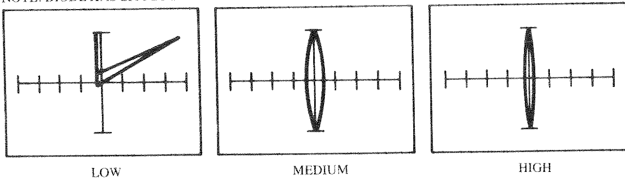
Figure 6-12. Tracker Display - Diode and a 1.0uF Capacitor
