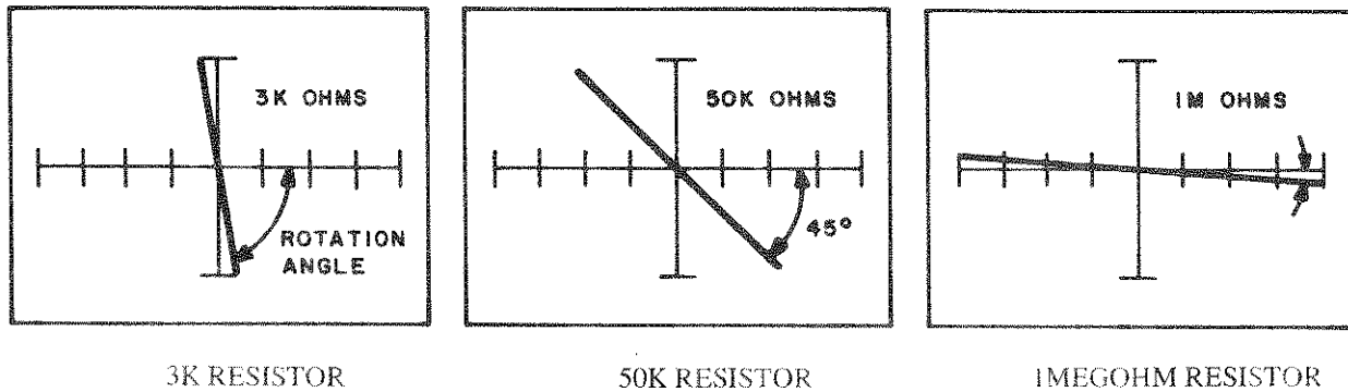
Figure 5-3. Effects of Resistor on Angle of Rotation - High Range
