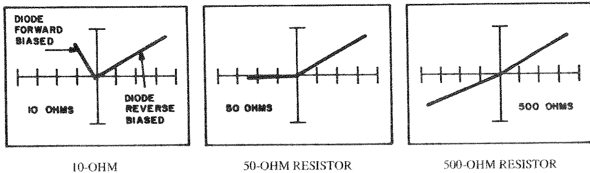
Figure 6-6. Low Range Patterns for Various Resistors and Series Diode
