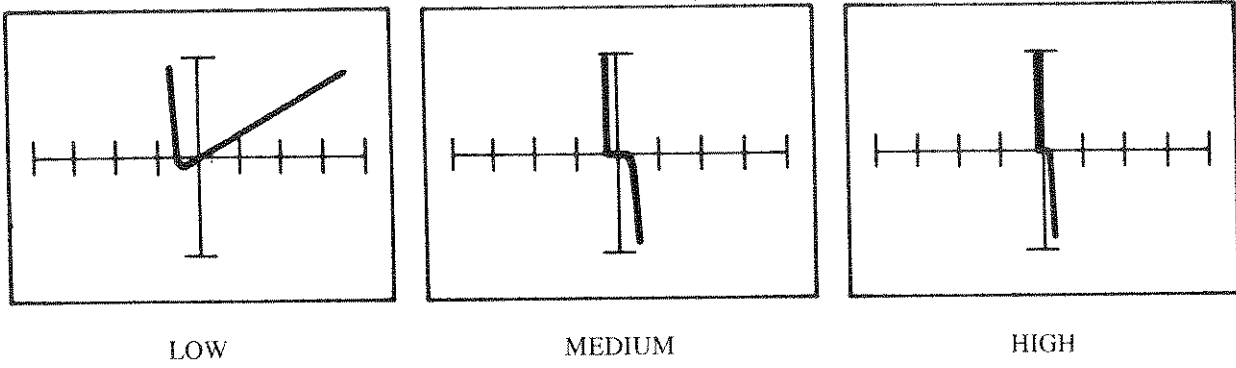
Figure 7-17. Patterns Between Input and Ground Pins - 7905
