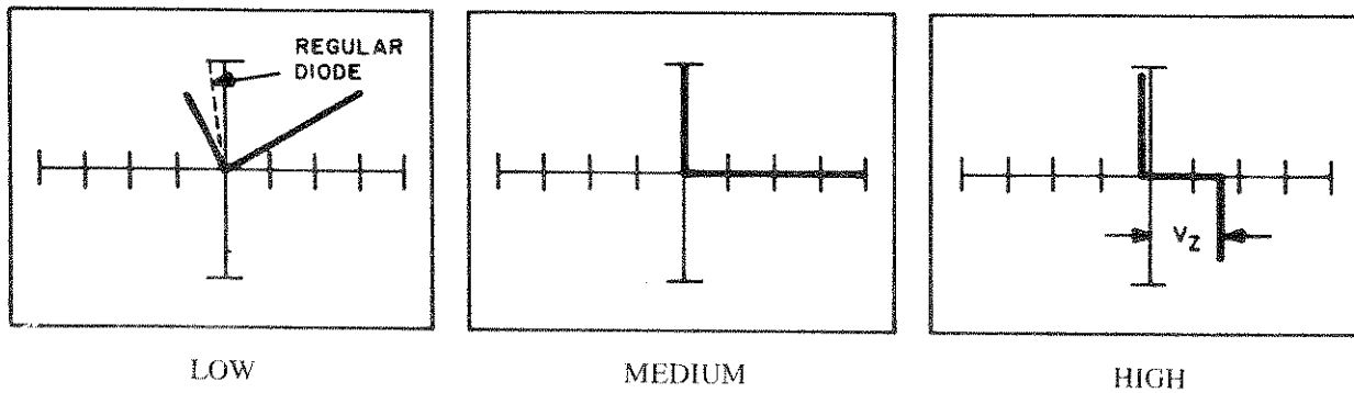
Figure 4-23. Gate-to-Source Patterns
