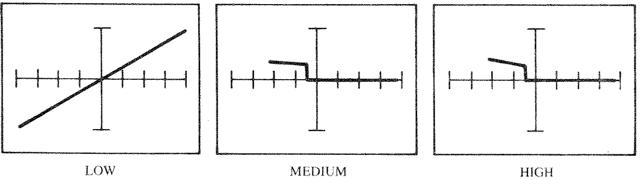
Figure 7-5. Patterns Between Pins 8 and 3 (V + and Non-Inverting Input)
