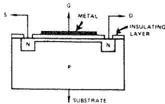
Idealized cross-section through an N-channel depletion-type MOSFET
