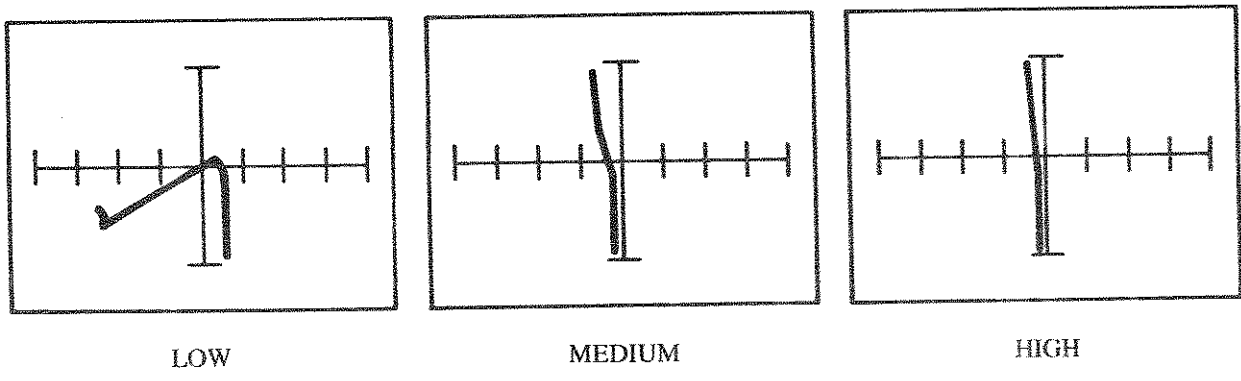
Figure 7-13. Patterns Between Output and Ground Pins - 7805
