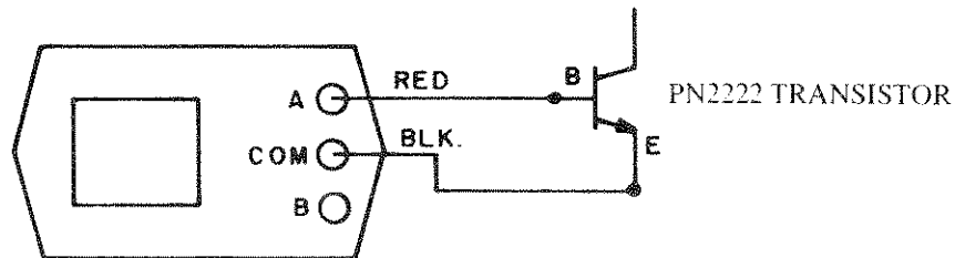
Figure 3-22. NPN Base-Emitter Junction Connections
