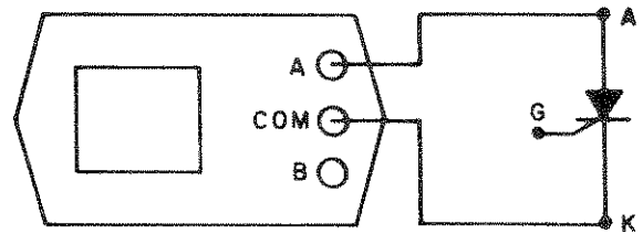
Figure 8-5. Anode and Cathode Test Connections
