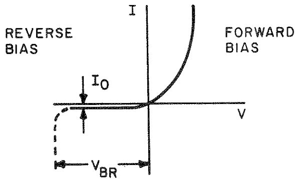
Figure 3-4. The Volt-Ampere Characteristic of a Semiconductor Diode
