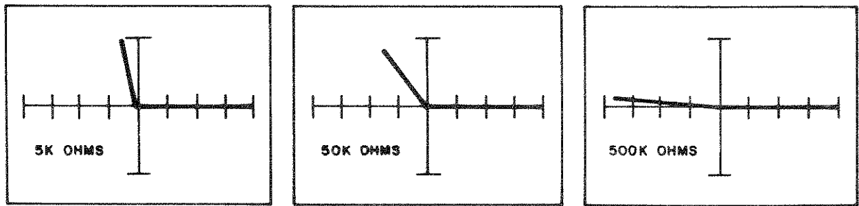
5K-OHM RESISTOR
