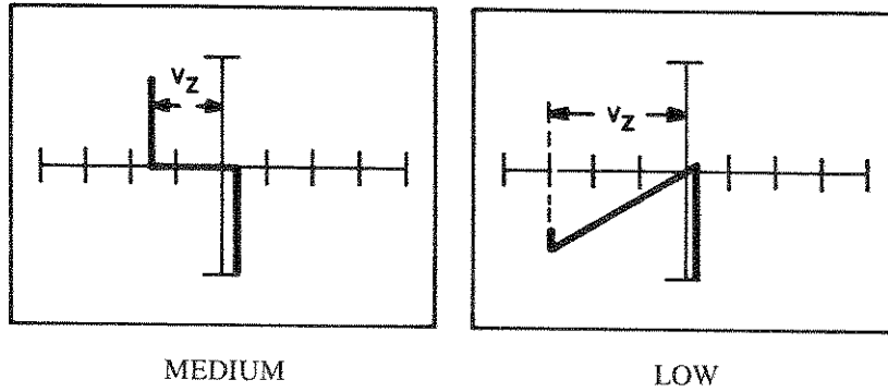
Figure 4-9. Pattern of B-E Connection - MPSA92 Transistor
