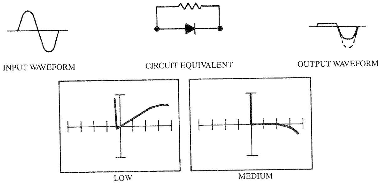
Figure 3-10. Waveforms and Typical Patterns - Leaky Diode
