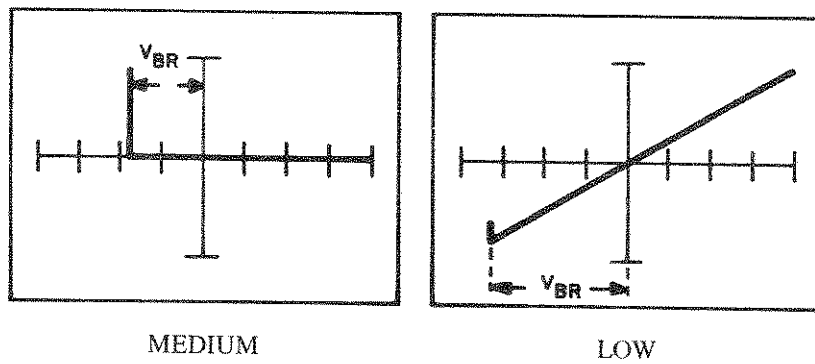
Figure 4-10. Pattern of C-E Connection - MPSA92 Transistor
