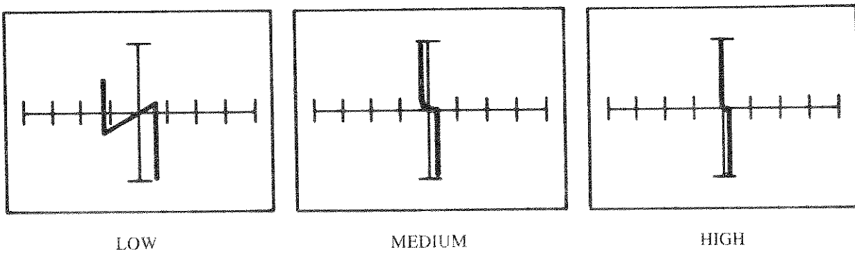
Figure 7-19. Patterns Between Input and Output Pins - 7905
