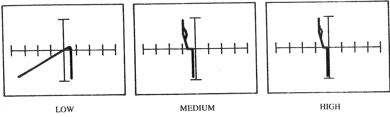
Figure 7-12. Patterns Between Input and Ground Pins - 7805
