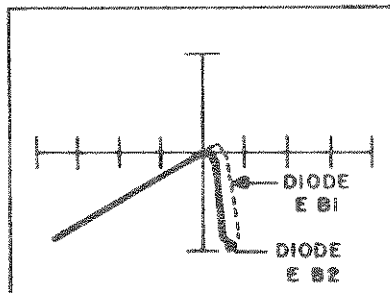
Figure 4-33. Low Range Pattern for Diodes E-B1 and E-B2
