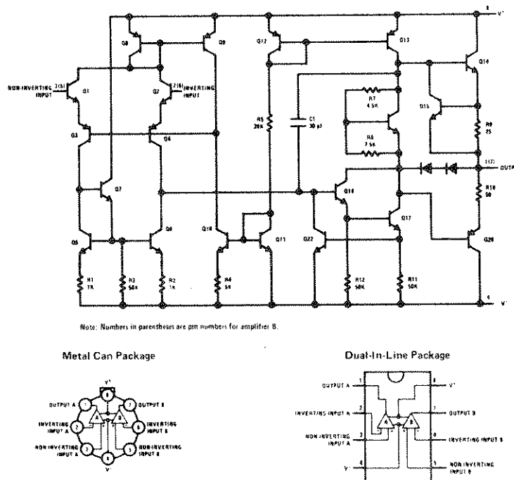
Figure 7-2. The LM-1458 Op-Amp. Schematic and Connections
