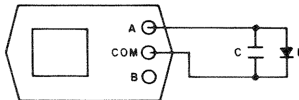
Figure 6-9. Test Circuit for Parallel Diode/Capacitor Combination
