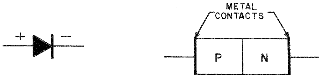
Figure 3-1. Diode Symbol
