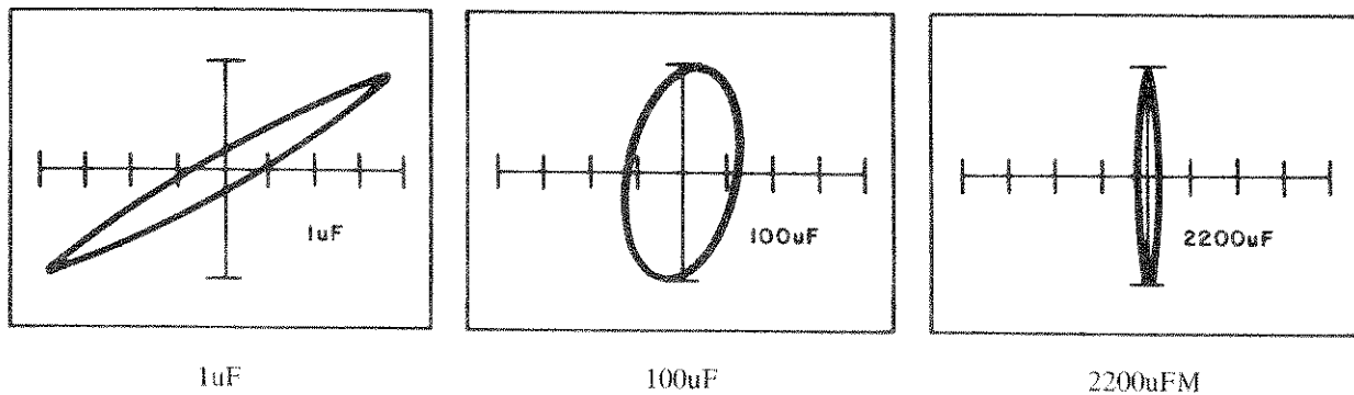
Figure 5-5. Capacitor Patterns Using the Low Range
