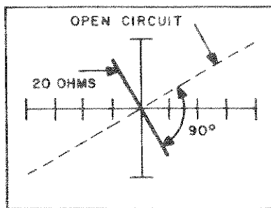
20-OHM RESISTOR
