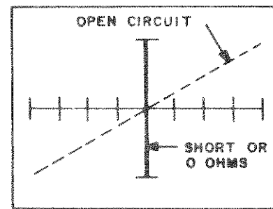
ZERO-OHM RESISTOR
