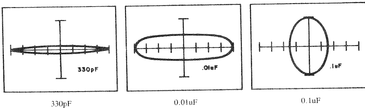
Figure 5-7. Capacitor Patterns Using the High Range
