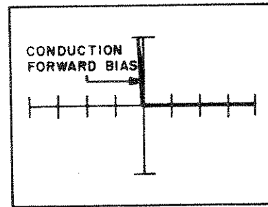
Figure 1-5. Trace of a Silicon Diode. Medium/High Range
