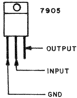
Figure 10-18. 7905 Pin Assignments
